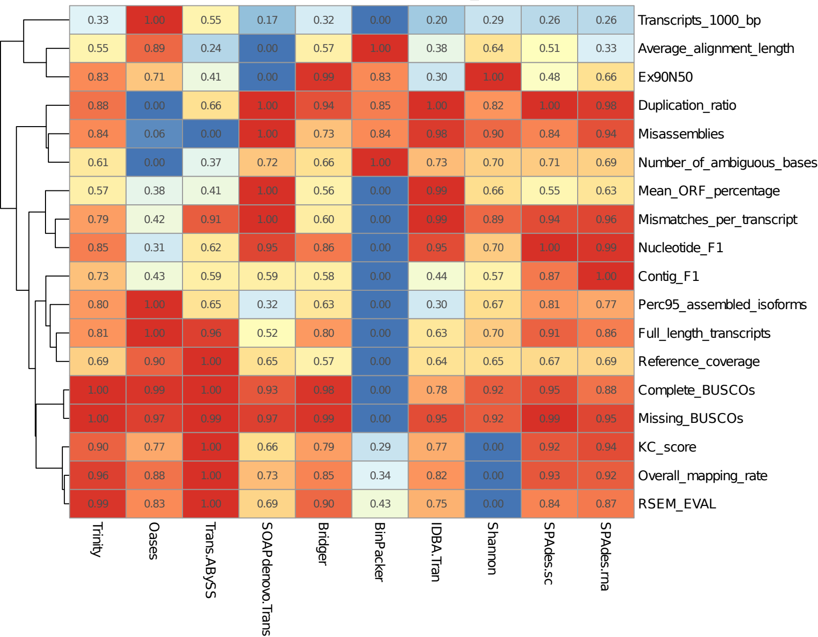
Metric (0,1)-norm. scores Arabidopsis_thaliana
