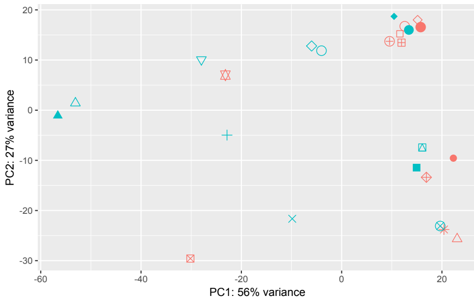
PC1 vs PC2: 24827 genes
