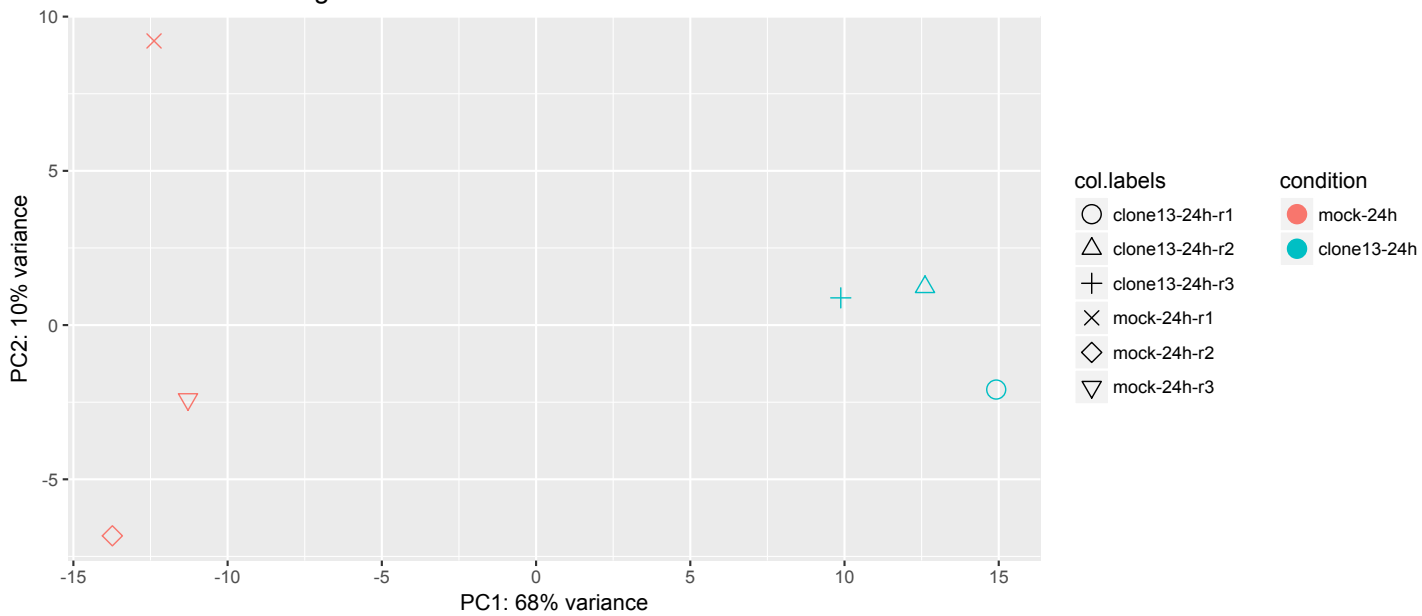
PC1 vs PC2: 24827 genes
