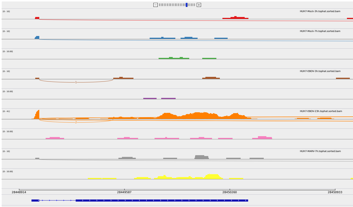
Figure 2: Sashimi plot of gene LOC401317.
