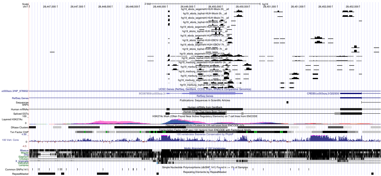
Figure 3: UCSC Genome Browser screenshot of gene LOC401317.
