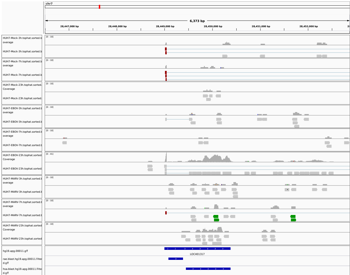
Figure 1: IGV Genome Browser screenshot of gene LOC401317.
