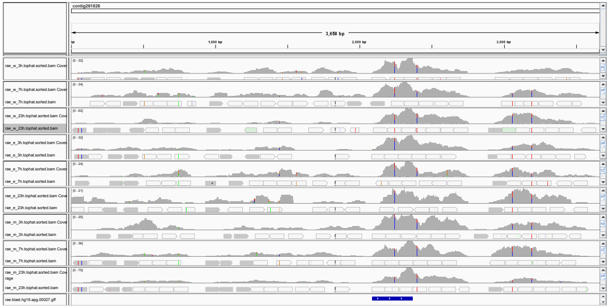
Figure 2: IGV Genome Browser screenshot of gene LMOD1 in bat.
