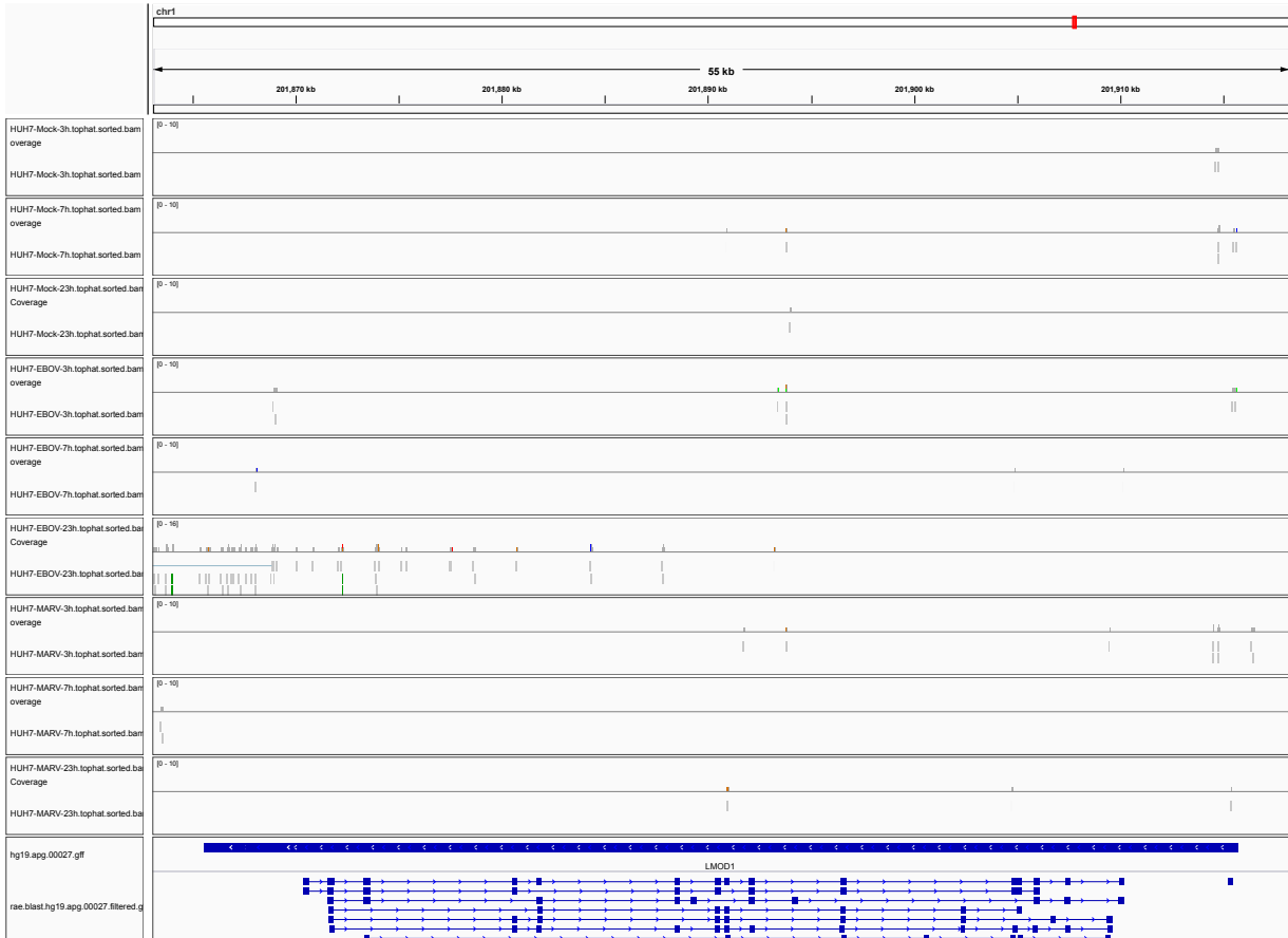
Figure 1: IGV Genome Browser screenshot of gene LMOD1.
