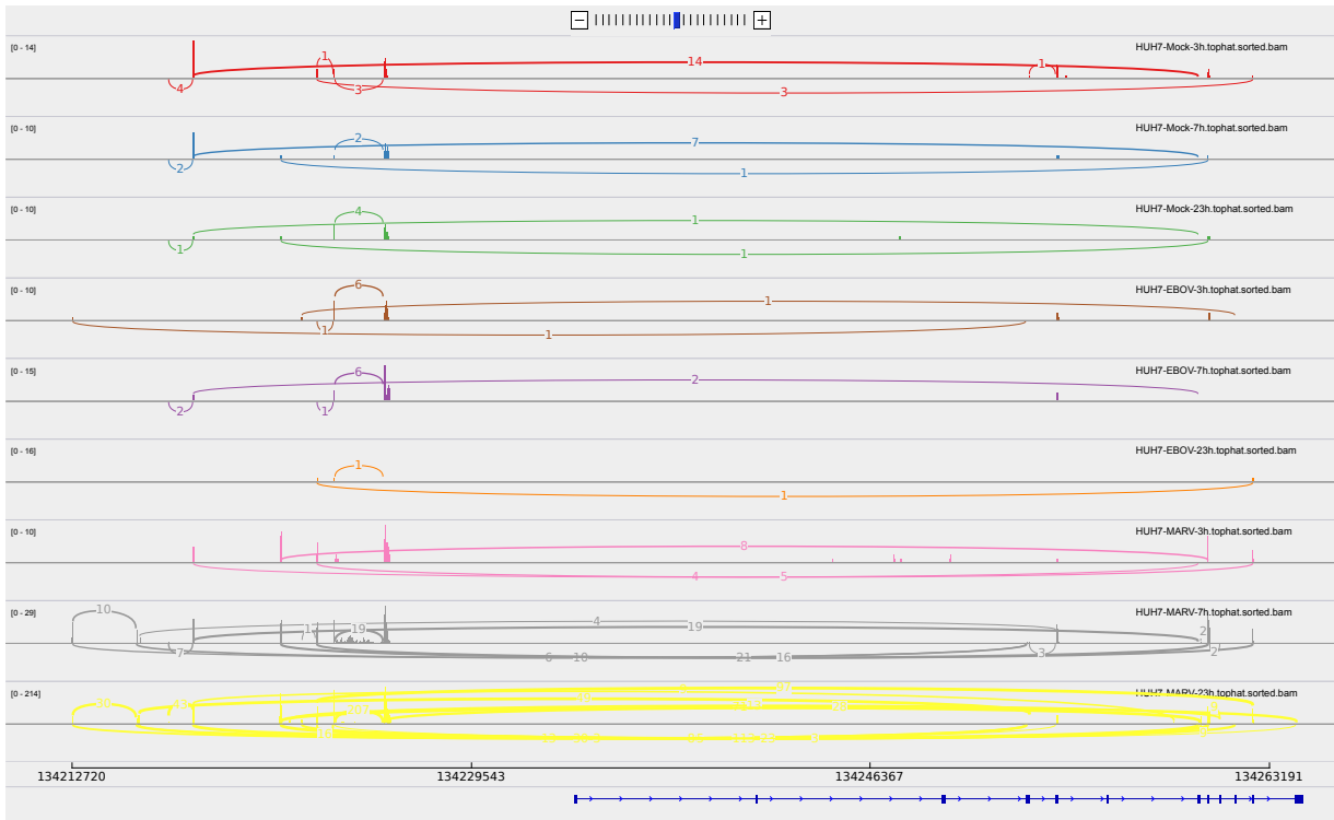
Figure 1: Sashimi plot of gene AKR1B15.
