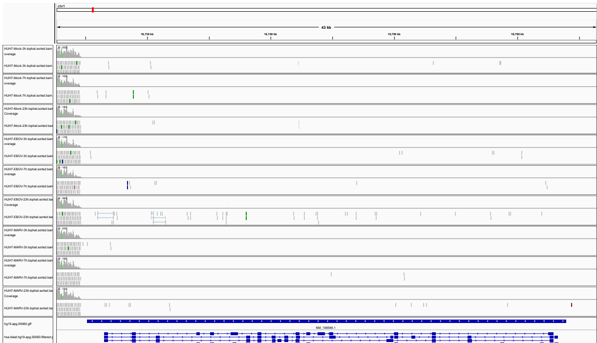
Figure 1: IGV Genome Browser screenshot of gene SPATA21.
