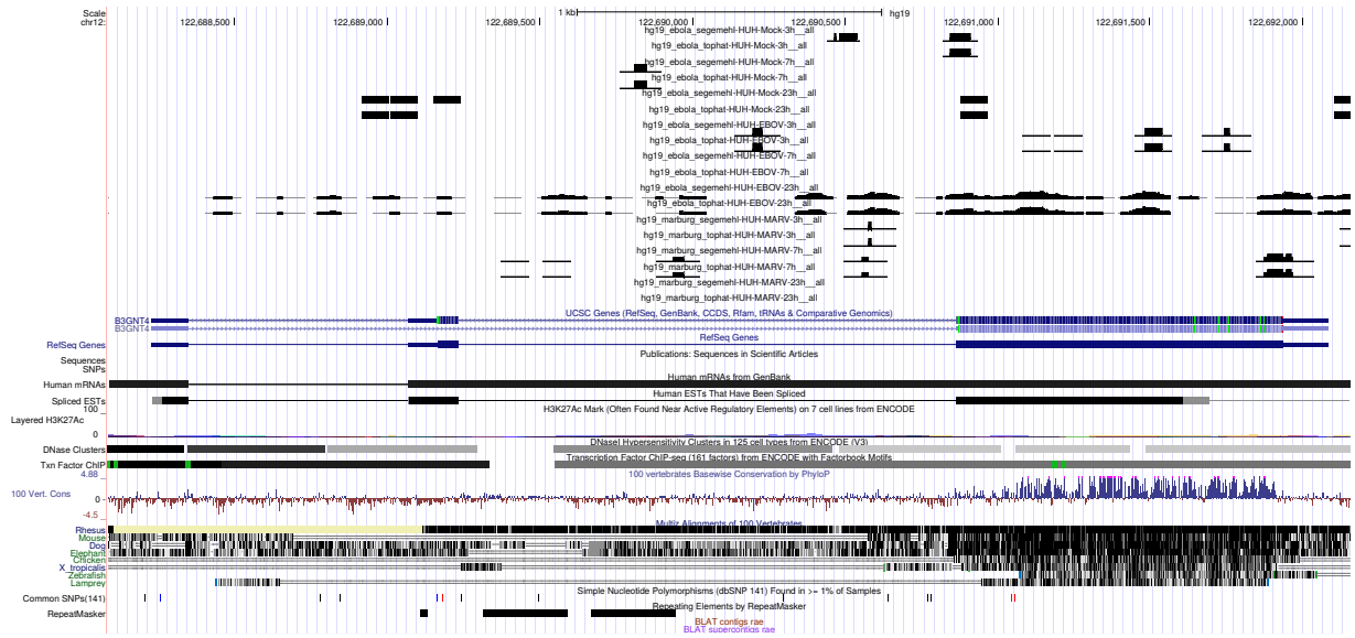
Figure 3: UCSC Genome Browser screenshot of gene B3GNT4.
