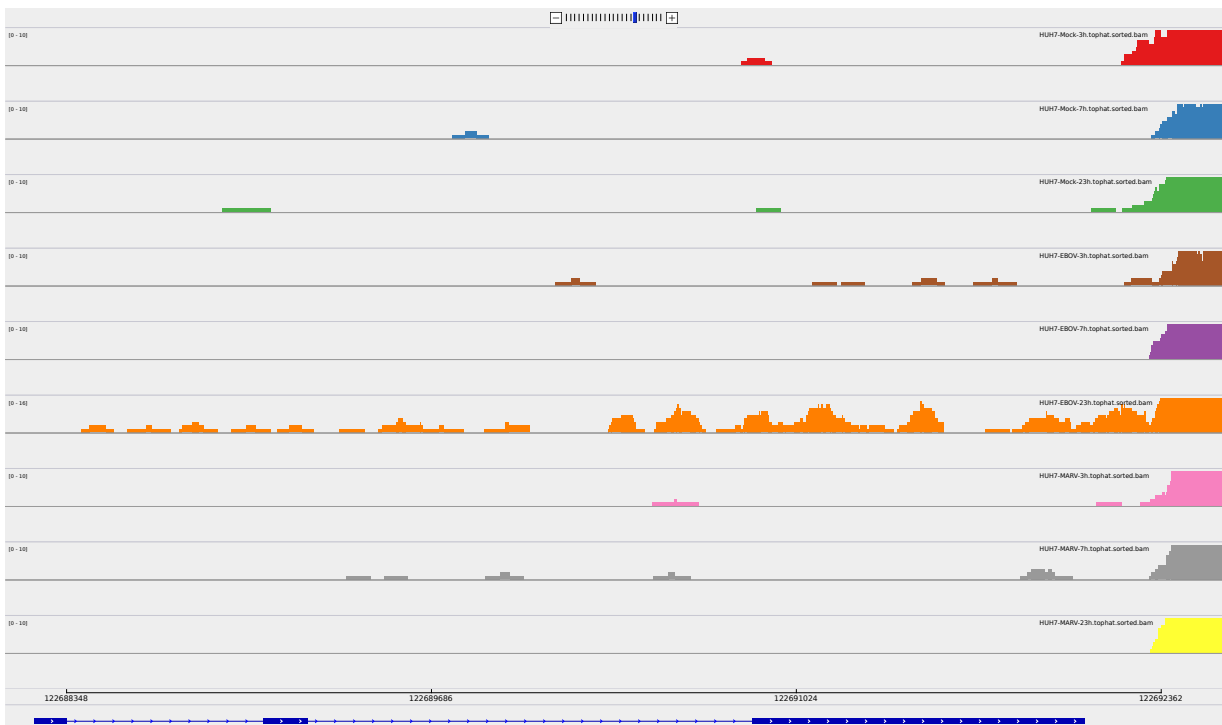
Figure 2: Sashimi plot of gene B3GNT4.
