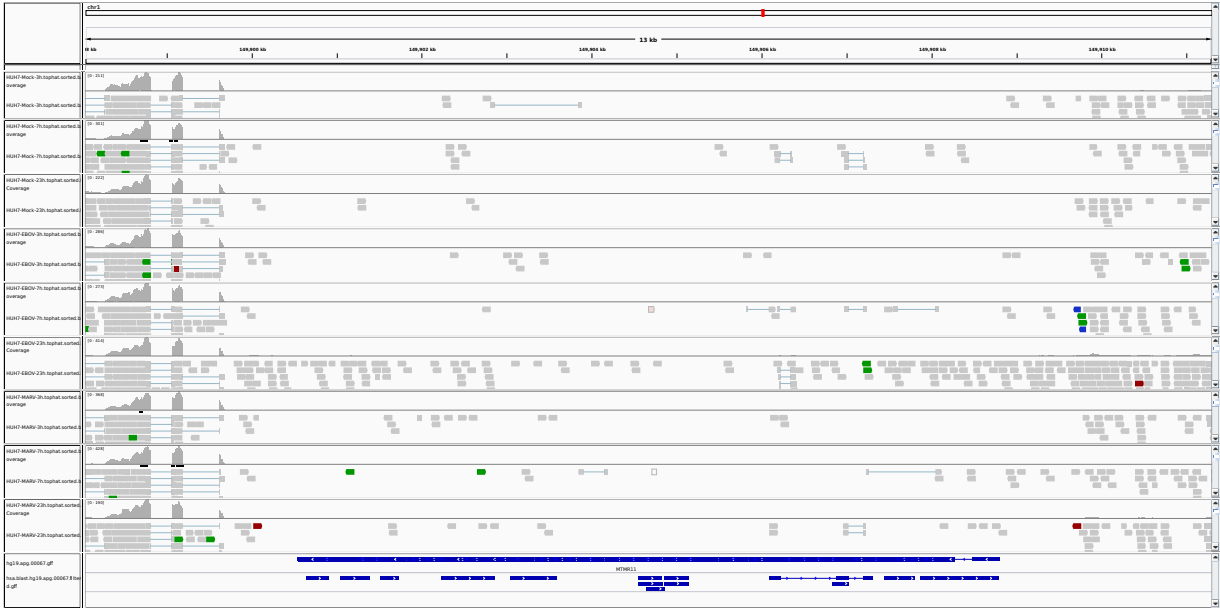
Figure 1: IGV Genome Browser screenshot of gene MTMR11.
