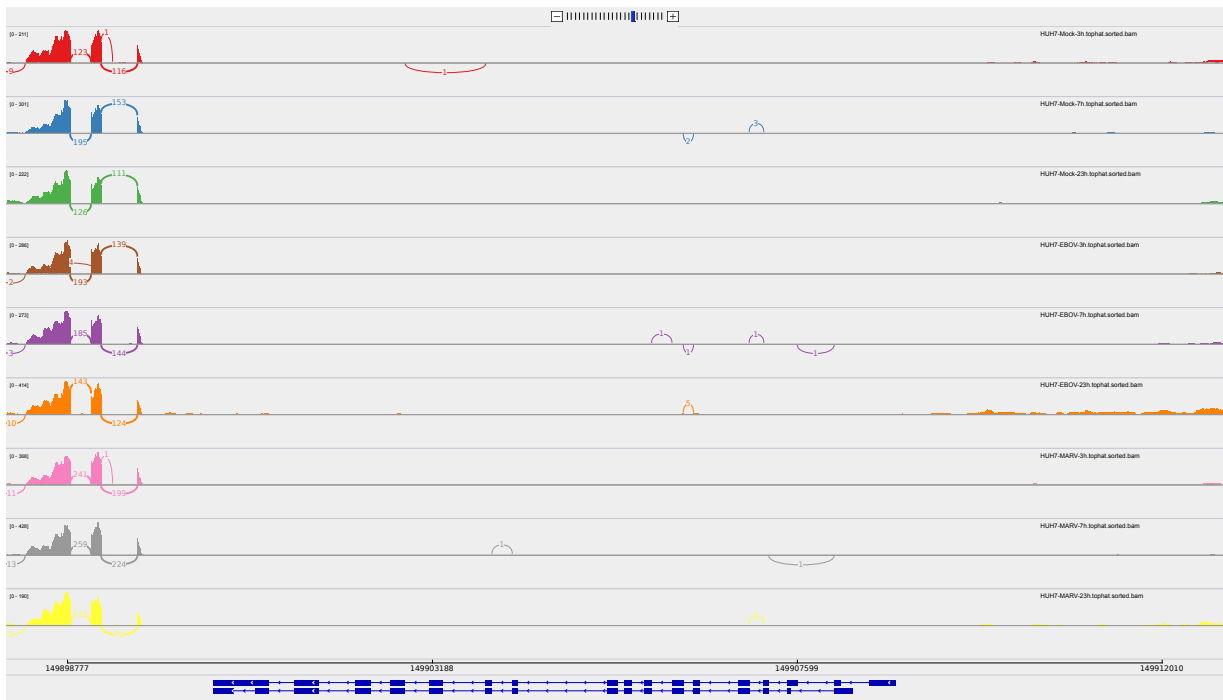
Figure 2: Sashimi plot of gene MTMR11.
