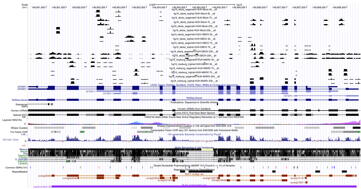
Figure 3: UCSC Genome Browser screenshot of gene MTMR11.
