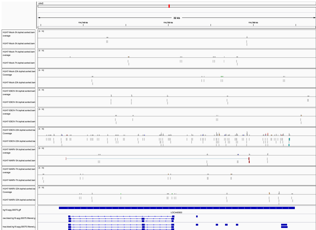
Figure 1: IGV Genome Browser screenshot of gene LOC440900.
