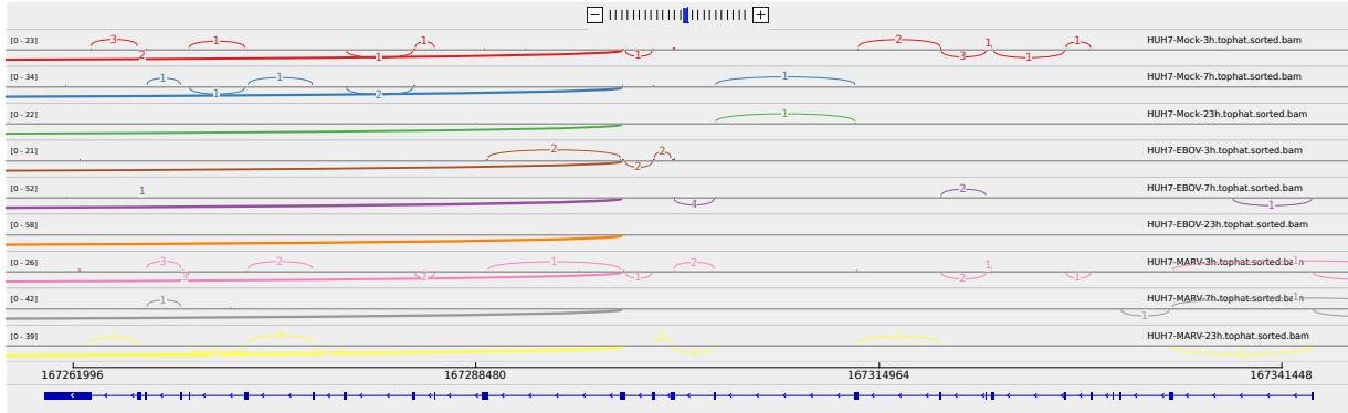
Figure 2: Sashimi plot of gene SCN7A.
