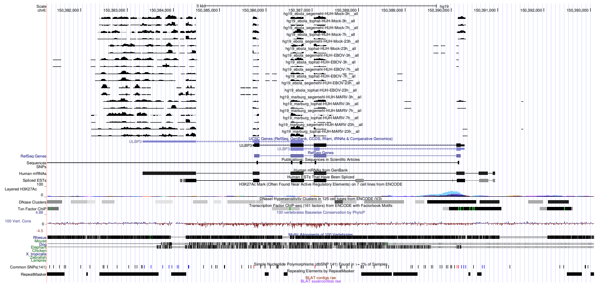
Figure 3: UCSC Genome Browser screenshot of gene ULBP3.
