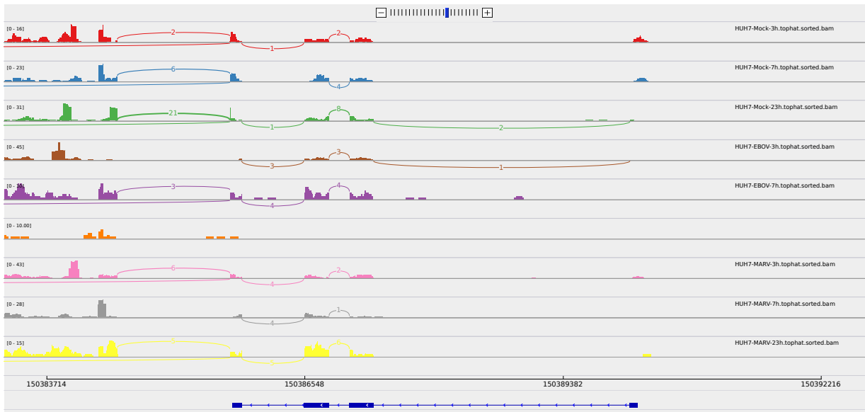
Figure 2: Sashimi plot of gene ULBP3.
