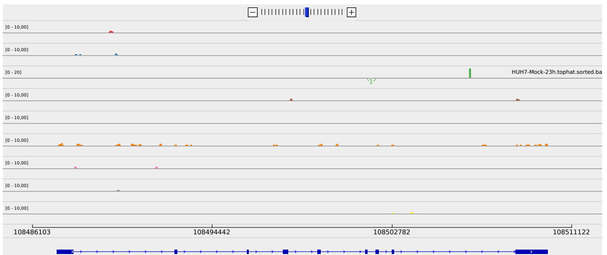
Figure 2: Sashimi plot of gene NR2E1.
