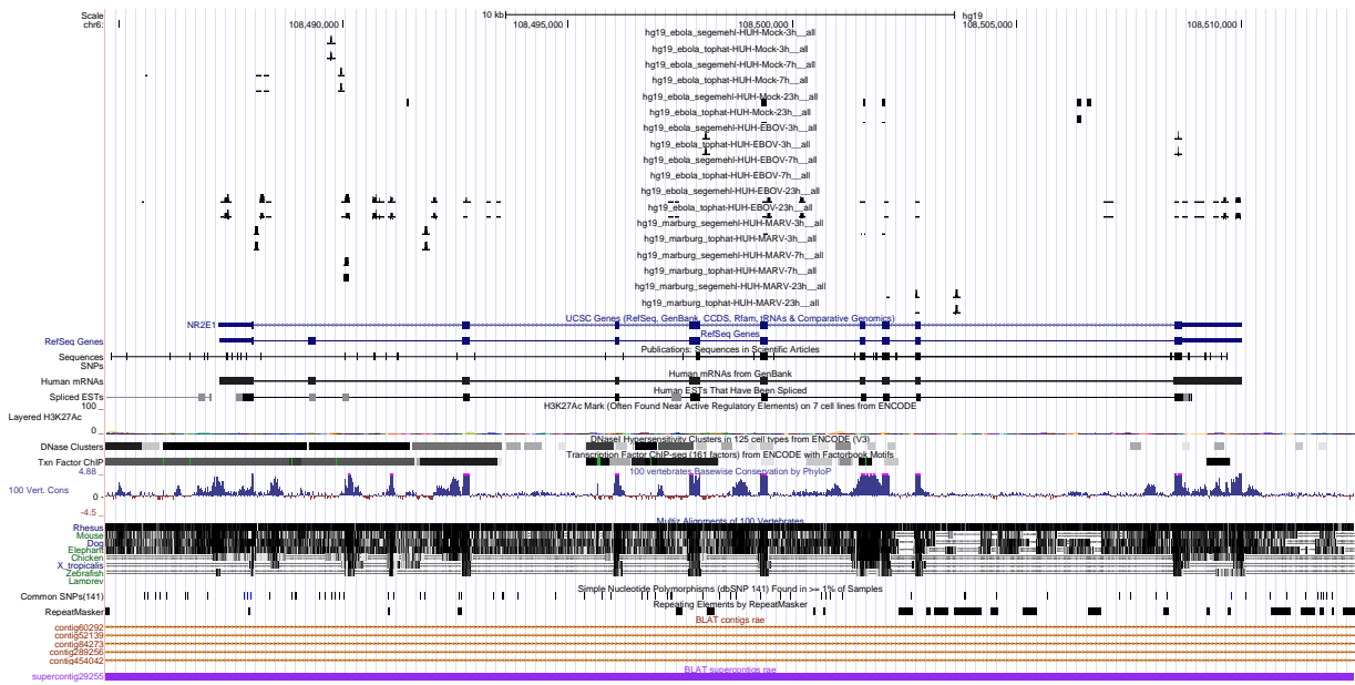
Figure 3: UCSC Genome Browser screenshot of gene NR2E1.
