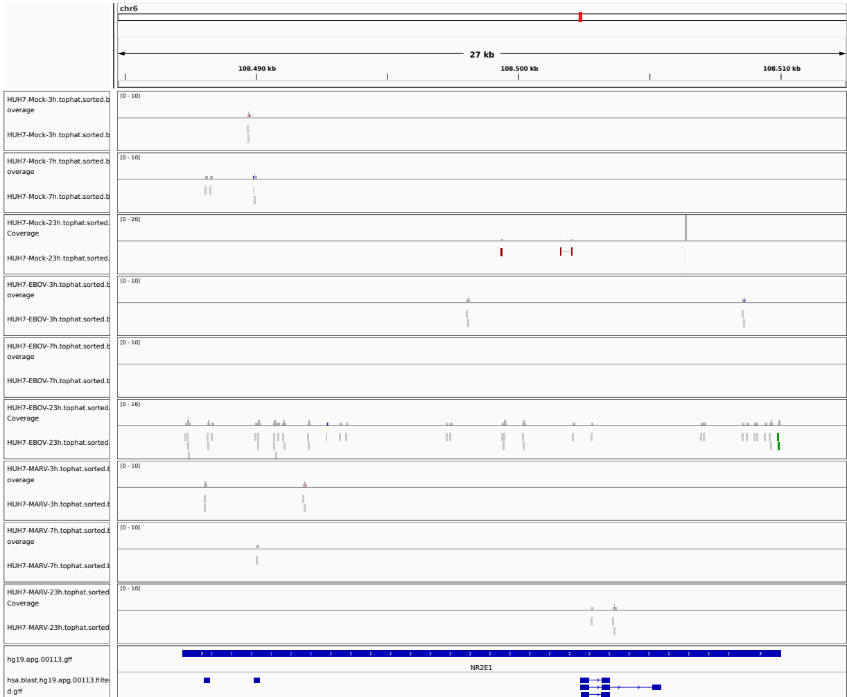
Figure 1: IGV Genome Browser screenshot of gene NR2E1.
