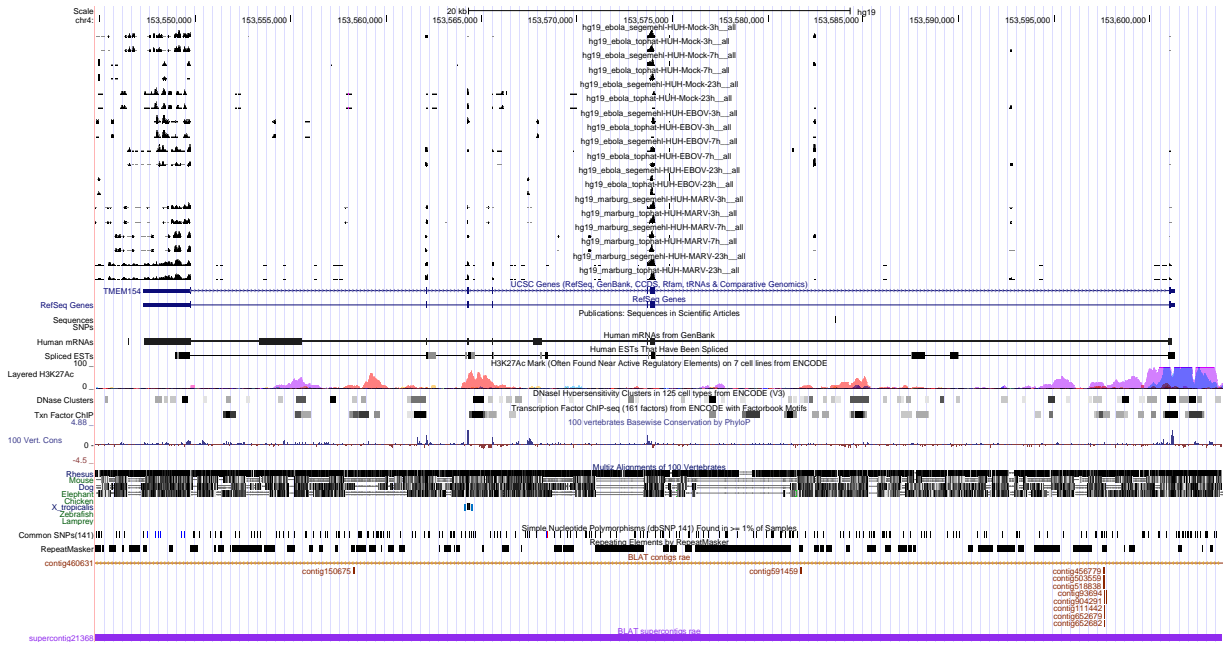
Figure 3: UCSC Genome Browser screenshot of gene TMEM154.
