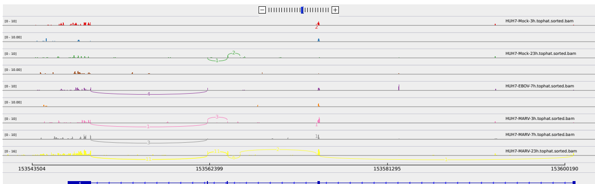
Figure 2: Sashimi plot of gene TMEM154.
