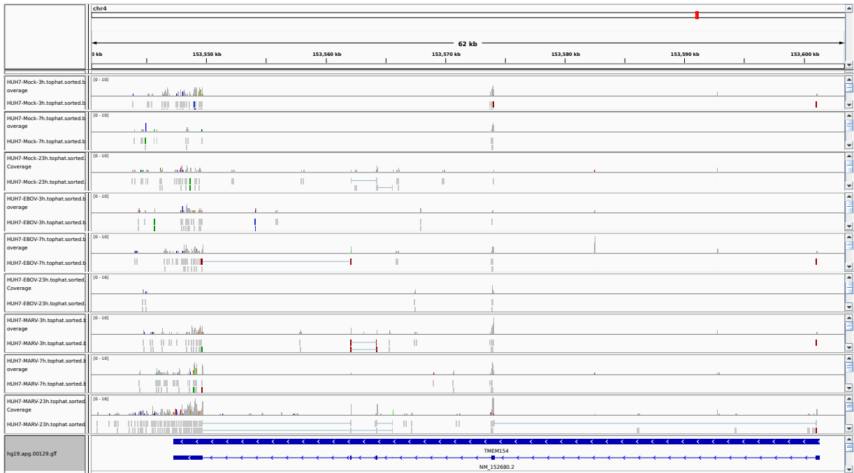
Figure 1: IGV Genome Browser screenshot of gene TMEM154.
