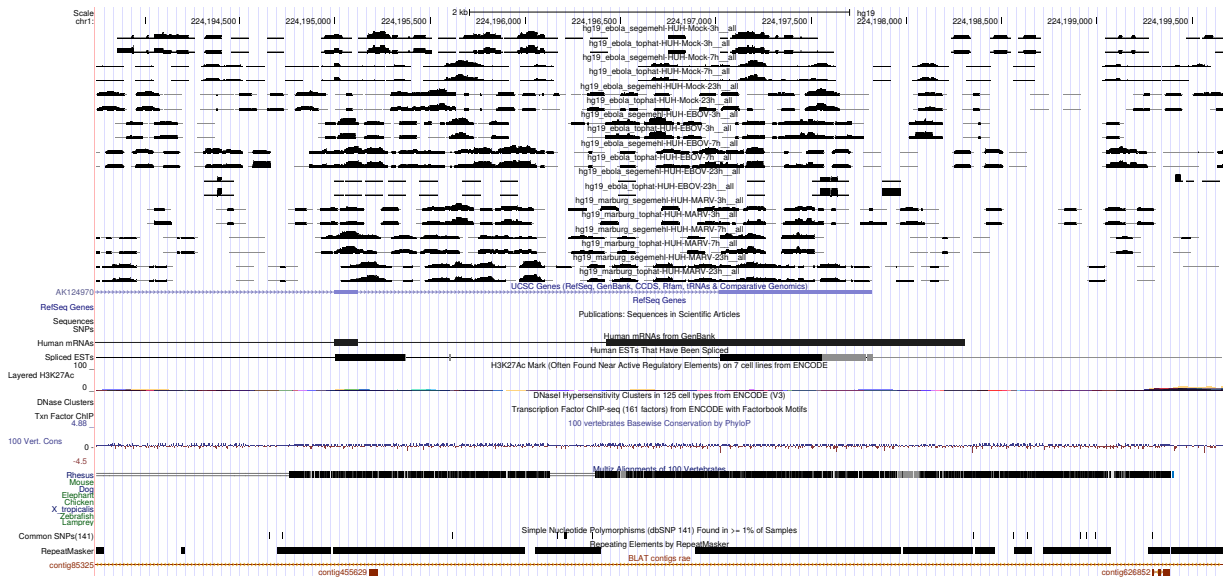
Figure 2: UCSC Genome Browser screenshot of gene LOC100287497.
