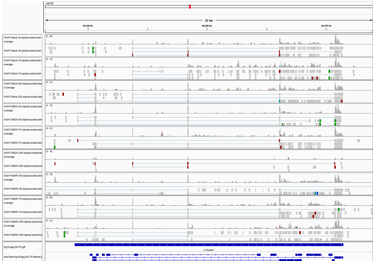
Figure 1: IGV Genome Browser screenshot of gene C15orf43.
