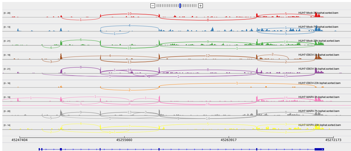
Figure 2: Sashimi plot of gene C15orf43.
