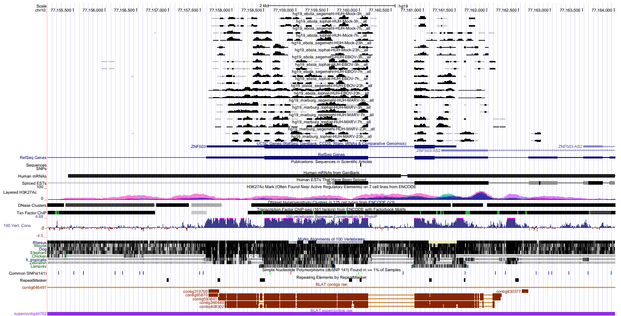
Figure 3: UCSC Genome Browser screenshot of gene ZNF503.
