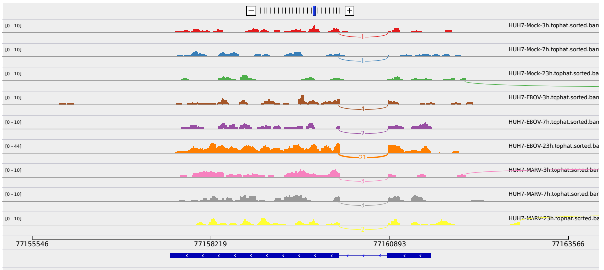
Figure 2: Sashimi plot of gene ZNF503.
