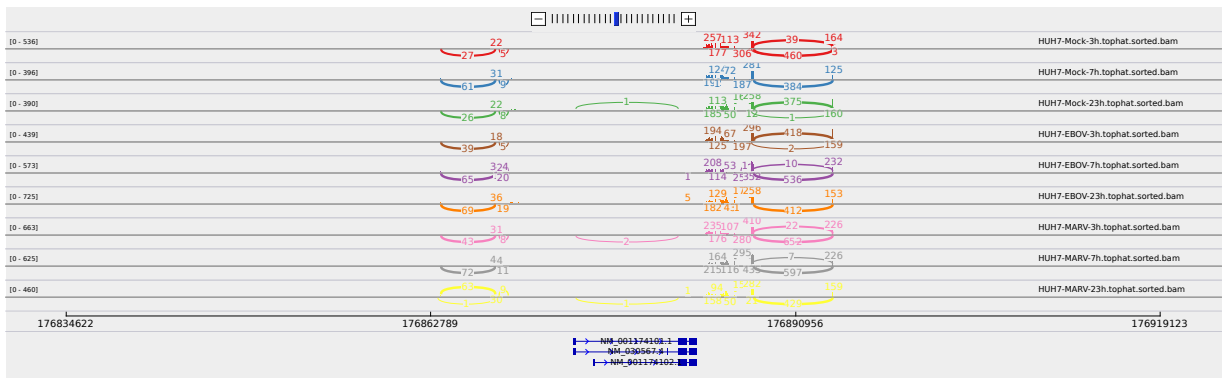
Figure 2: Sashimi plot of gene PRR7.
