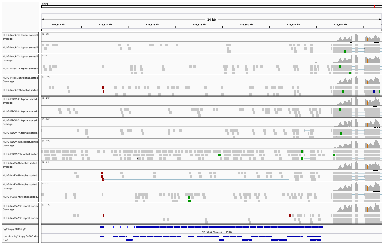
Figure 1: IGV Genome Browser screenshot of gene PRR7.
