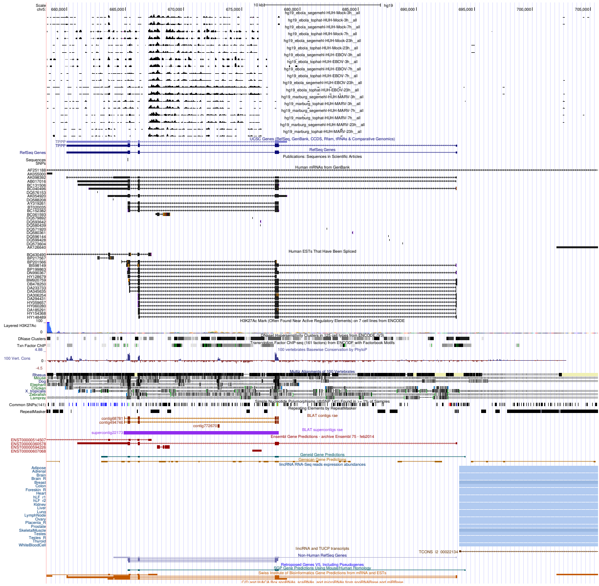
Figure 2: UCSC Genome Browser screenshot of gene TPPP.
