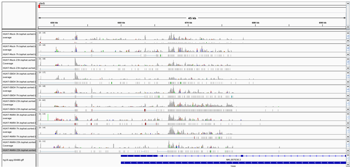
Figure 1: IGV Genome Browser screenshot of gene TPPP.
