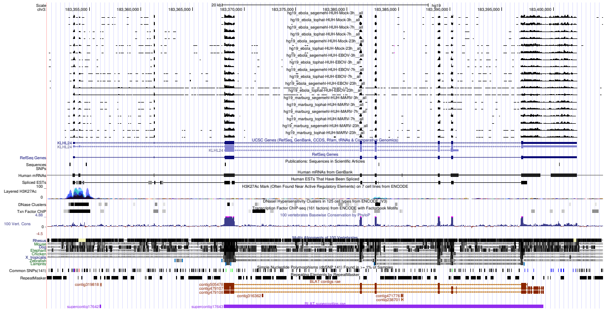
Figure 3: UCSC Genome Browser screenshot of gene KLHL24.
