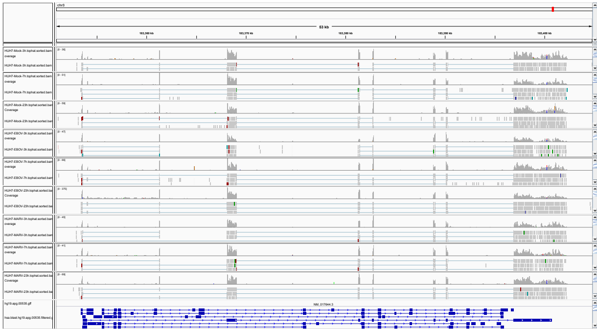
Figure 1: IGV Genome Browser screenshot of gene KLHL24.
