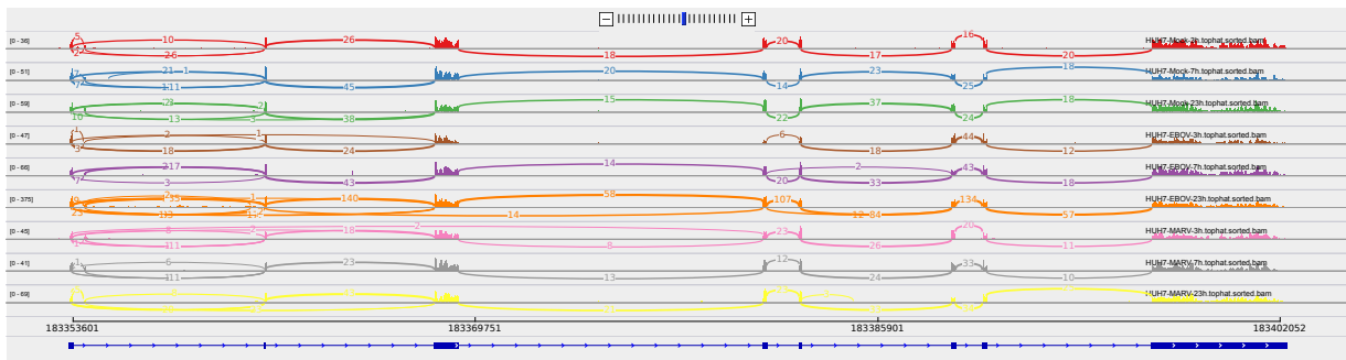
Figure 2: Sashimi plot of gene KLHL24.
