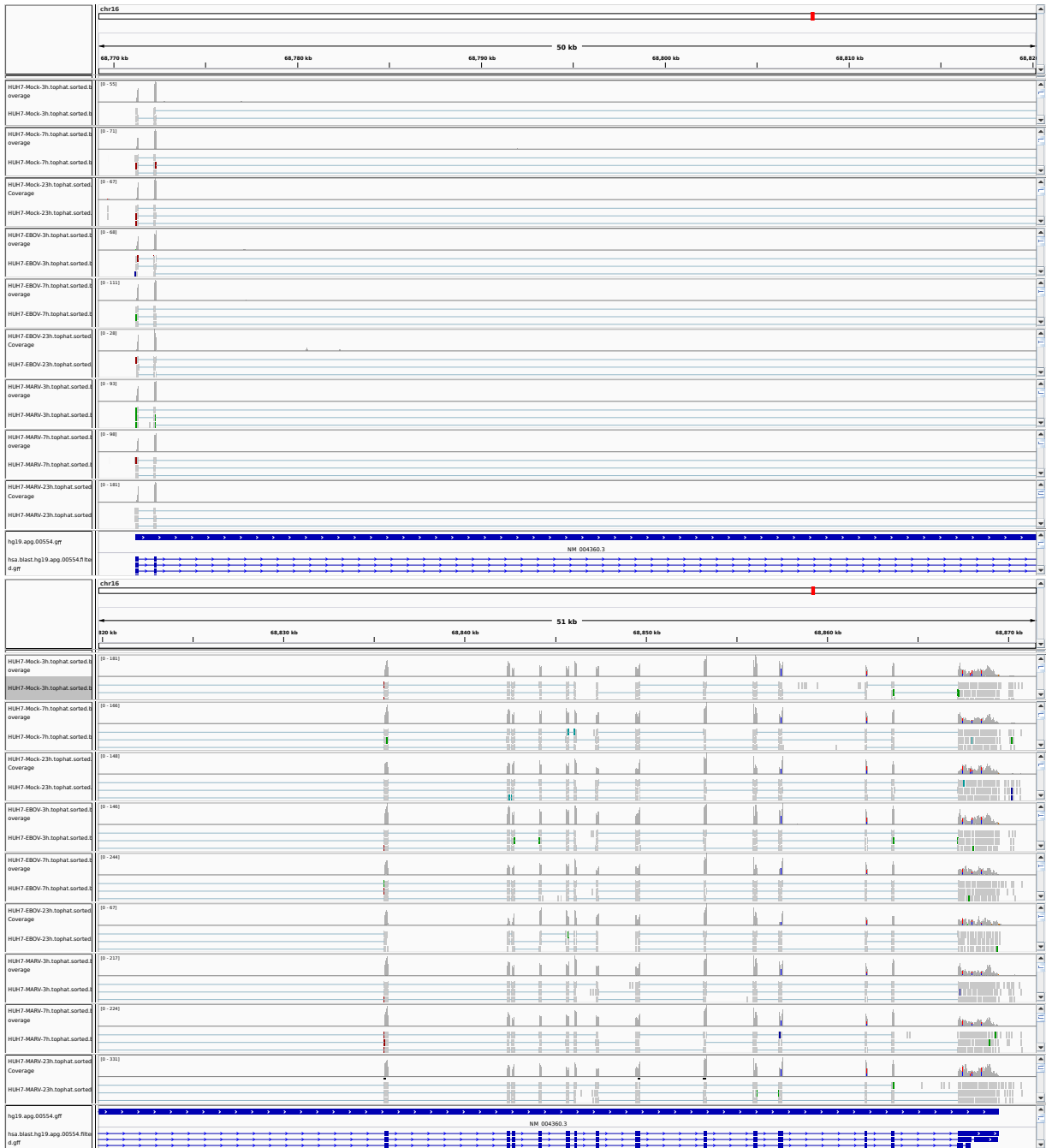
Figure 1: IGV Genome Browser screenshot of gene CDH1.
