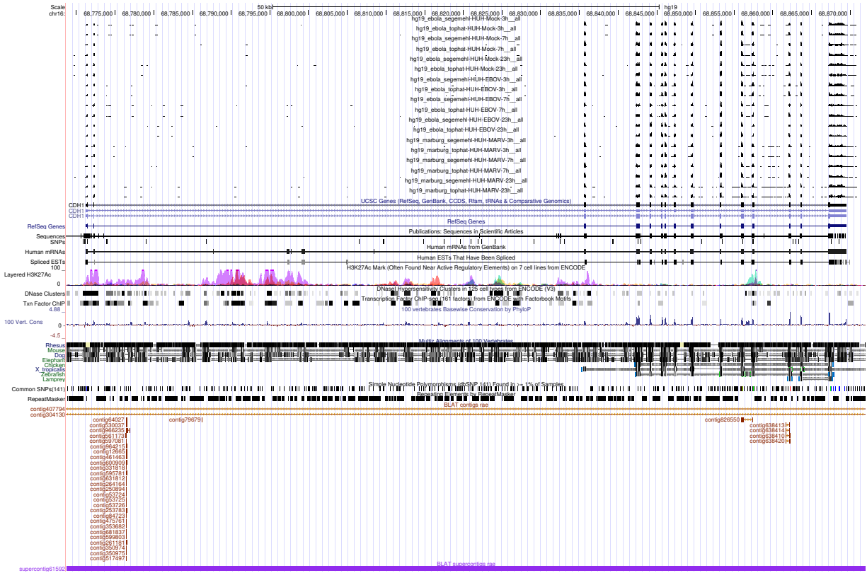
Figure 3: UCSC Genome Browser screenshot of gene CDH1.
