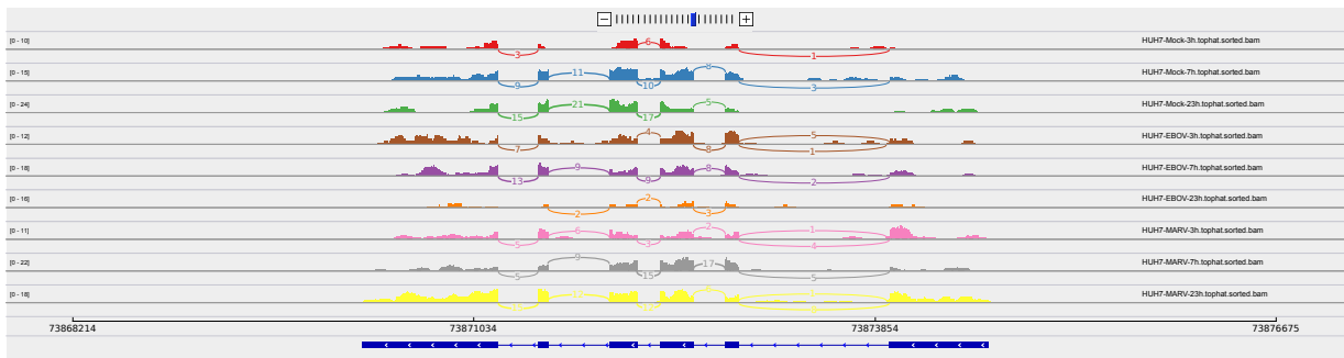
Figure 2: Sashimi plot of gene TRIM47.
