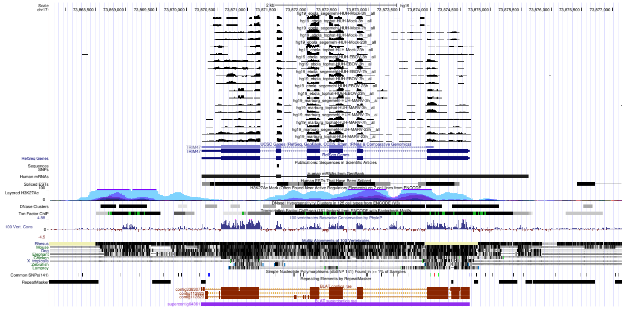
Figure 3: UCSC Genome Browser screenshot of gene TRIM47.
