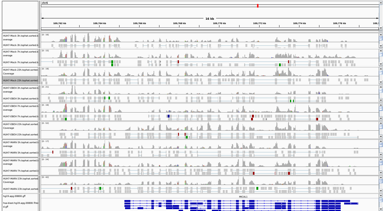
Figure 1: IGV Genome Browser screenshot of gene MICAL1.
