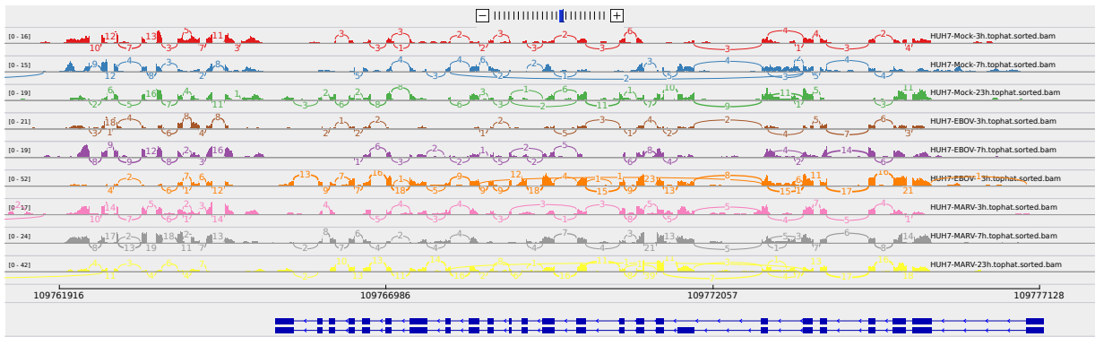
Figure 2: Sashimi plot of gene MICAL1.
