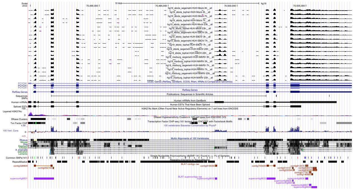
Figure 3: UCSC Genome Browser screenshot of gene PCYOX1.
