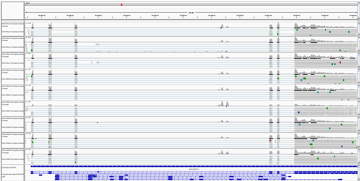
Figure 1: IGV Genome Browser screenshot of gene PCYOX1.
