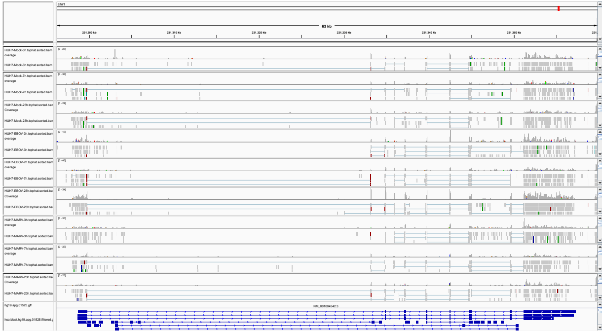
Figure 1: IGV Genome Browser screenshot of gene TRIM67.
