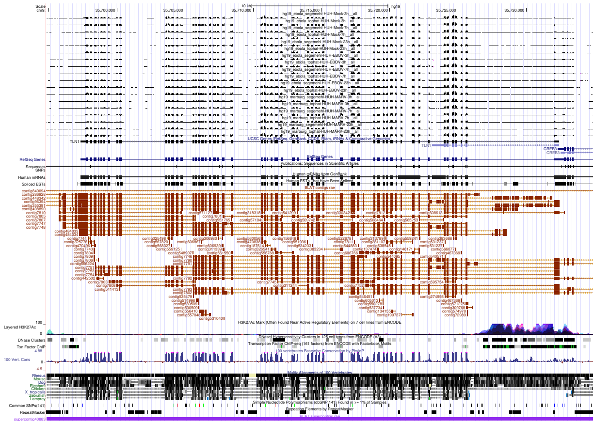
Figure 3: UCSC Genome Browser screenshot of gene TLN1.
