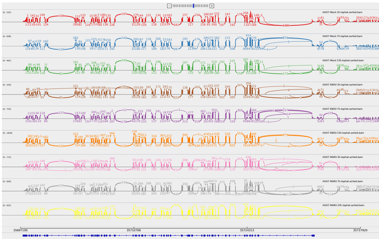
Figure 2: Sashimi plot of gene TLN1.
