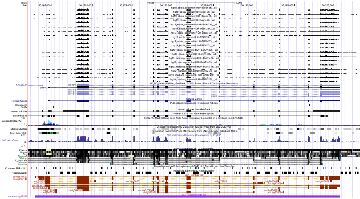
Figure 6: UCSC Genome Browser screenshot of gene BRPF3.
