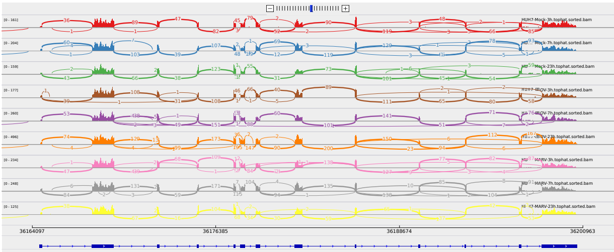
Figure 3: Sashimi plot of gene BRPF3.
