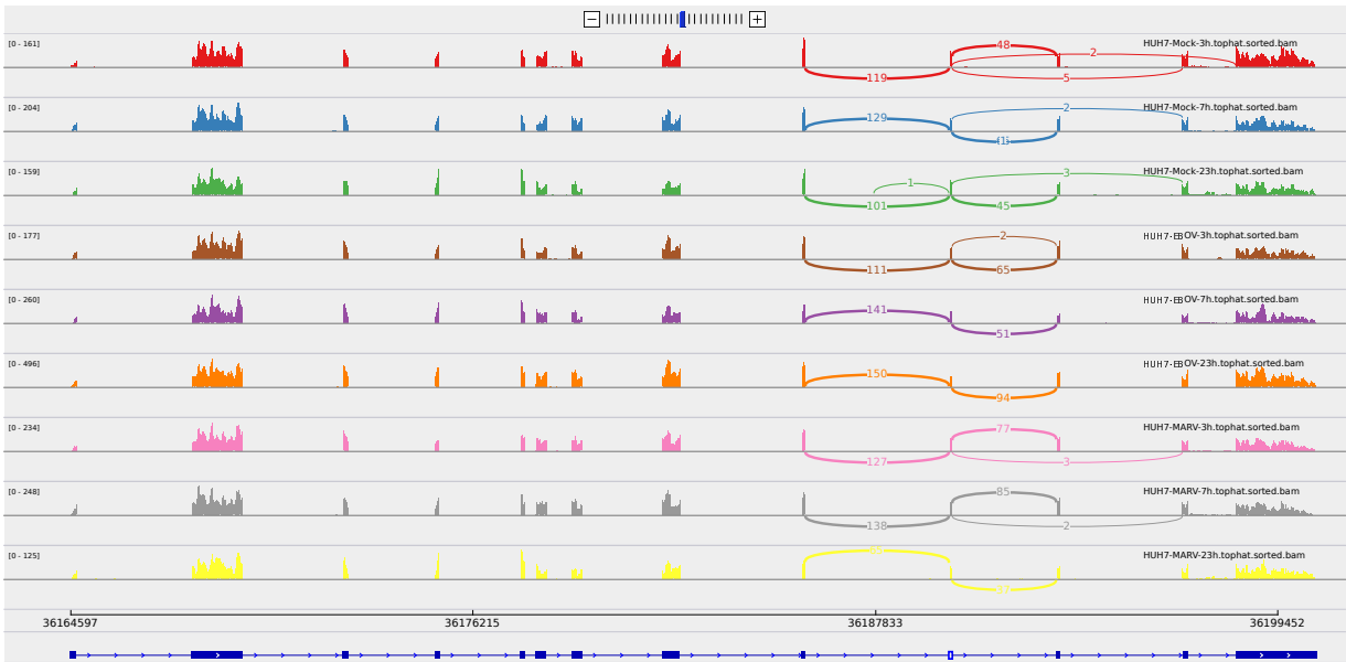
Figure 4: Sashimi plot of gene BRPF3.
