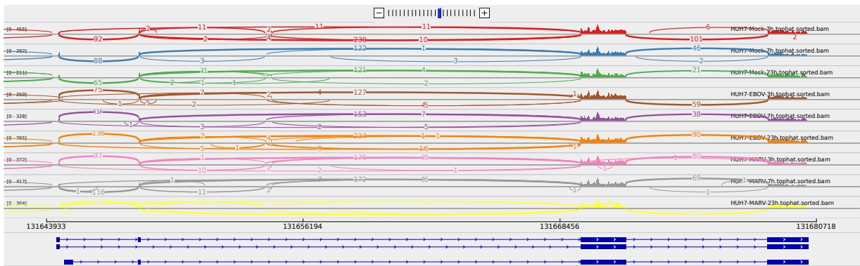
Figure 2: Sashimi plot of gene LRRC8A.
