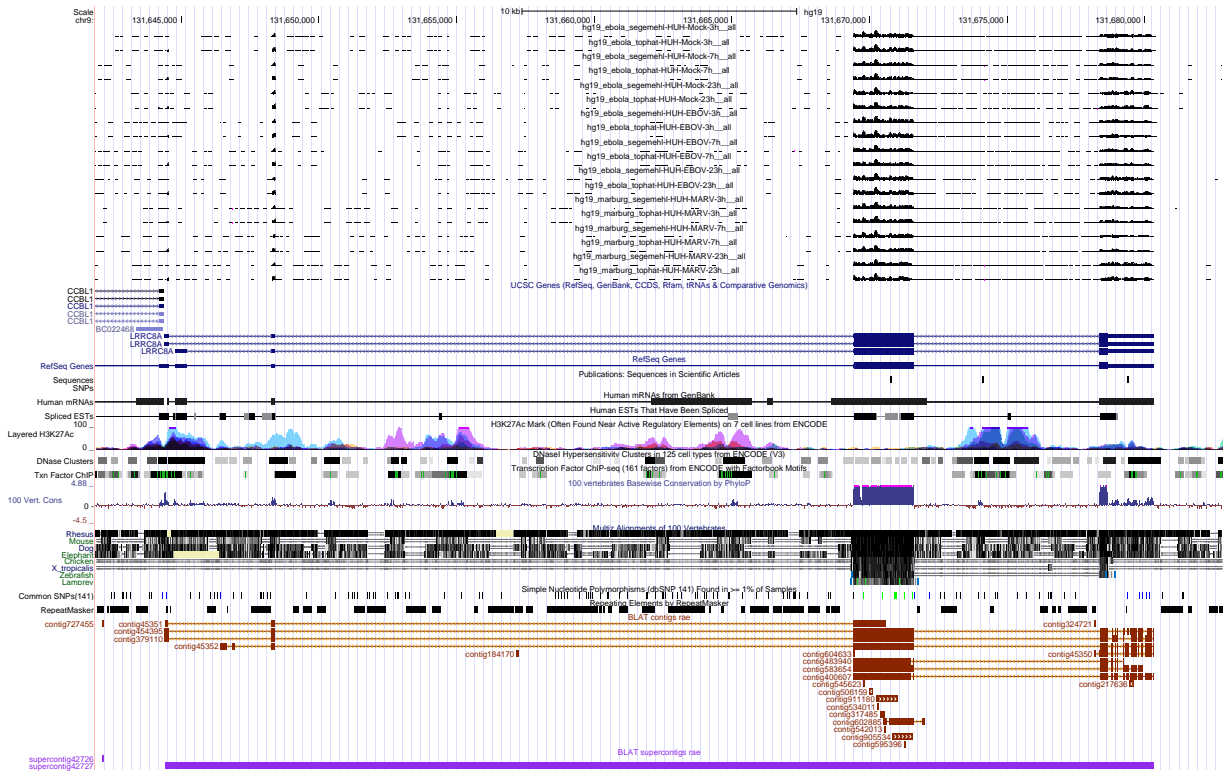
Figure 4: UCSC Genome Browser screenshot of gene LRRC8A.
