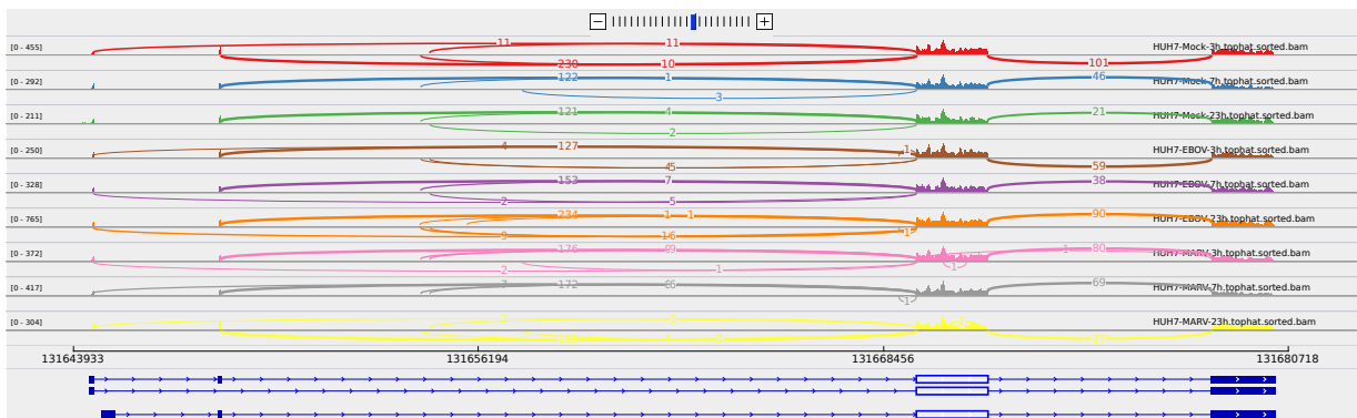
Figure 3: Sashimi plot of gene LRRC8A.
