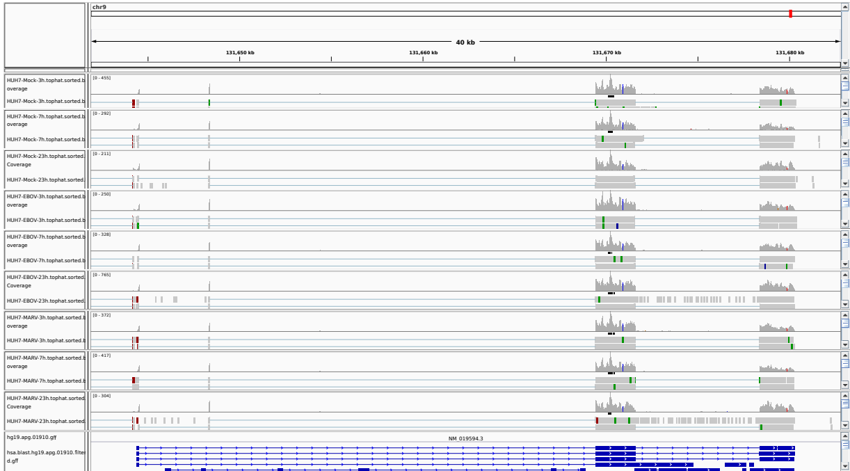
Figure 1: IGV Genome Browser screenshot of gene LRRC8A.
