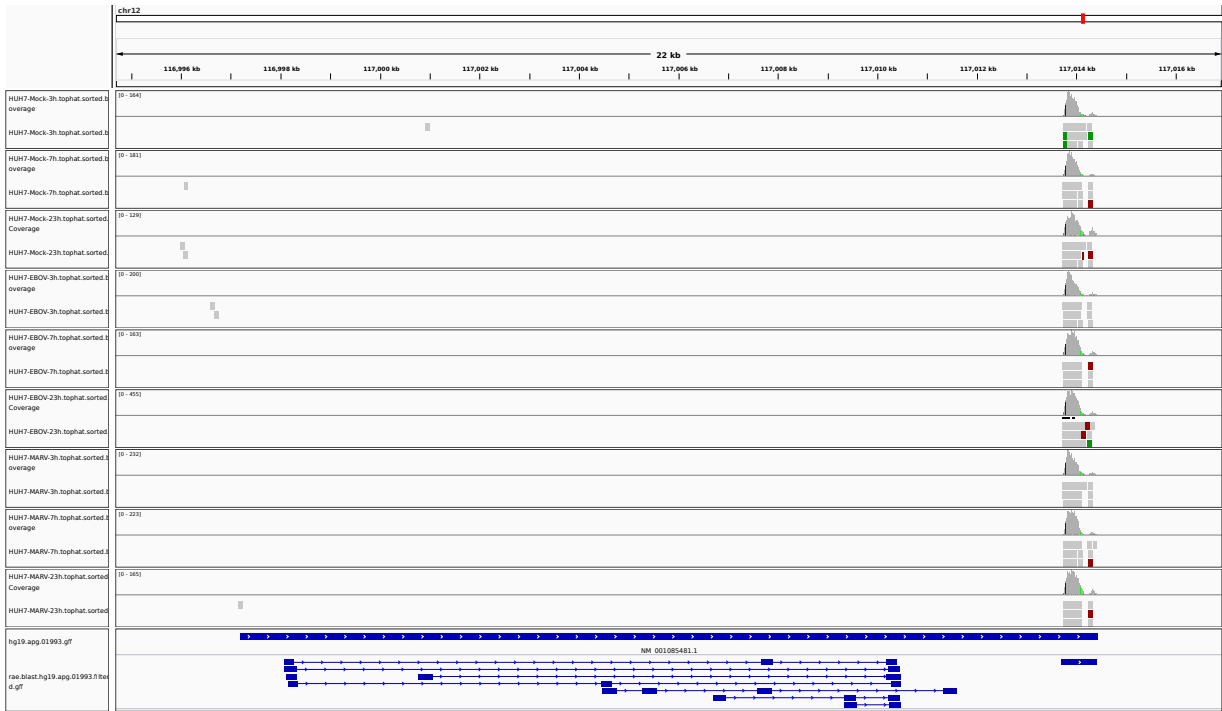
Figure 1: IGV Genome Browser screenshot of gene MAP1LC3B2.
