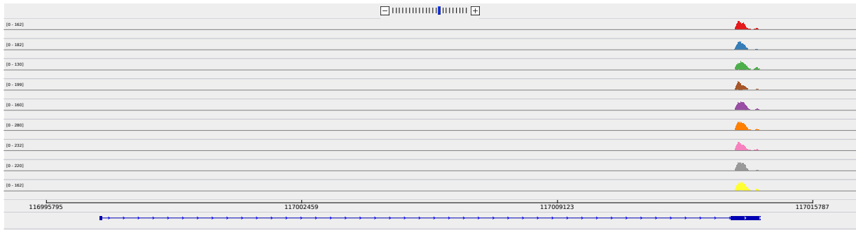
Figure 2: Sashimi plot of gene MAP1LC3B2.
