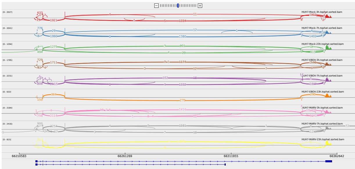
Figure 2: Sashimi plot of gene HMGA2.
