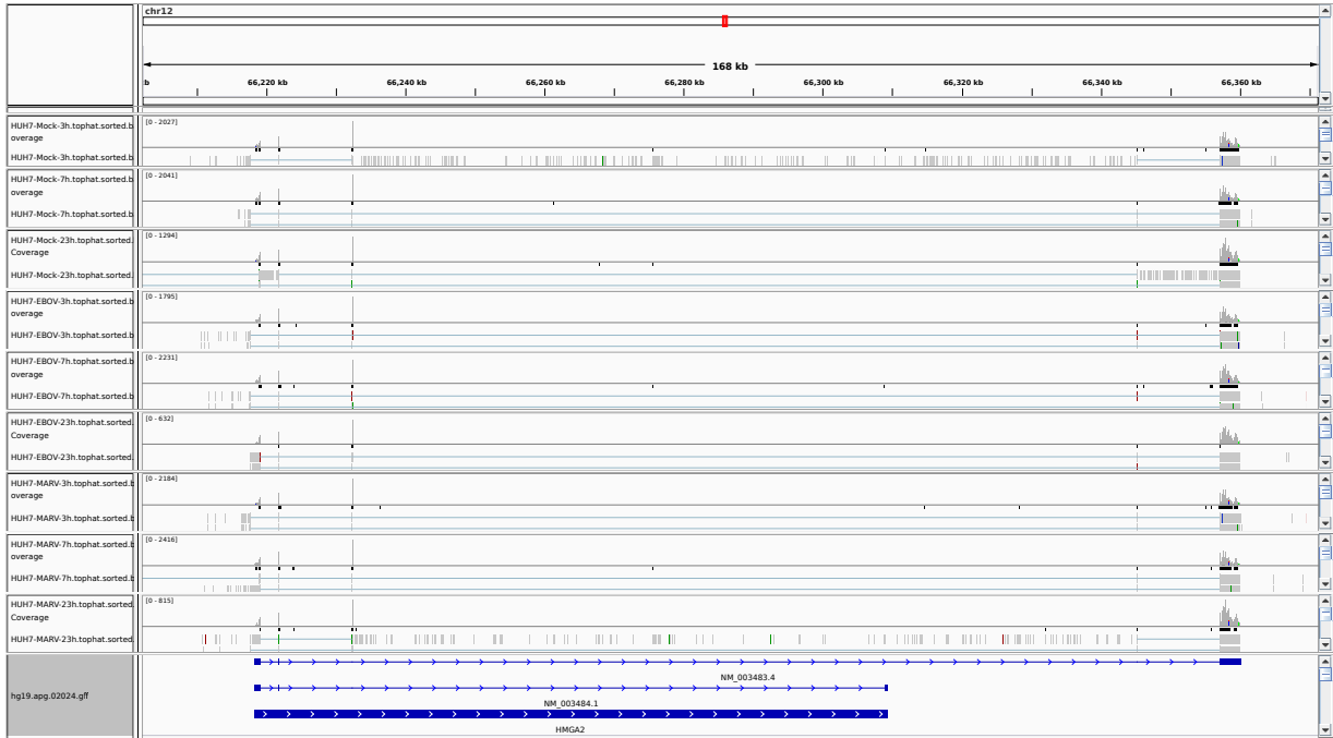
Figure 1: IGV Genome Browser screenshot of gene HMGA2.
