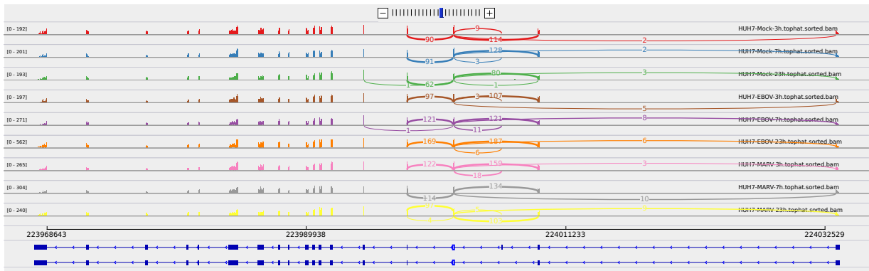
Figure 4: Sashimi plot of gene TP53BP2.
