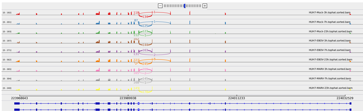
Figure 3: Sashimi plot of gene TP53BP2.
