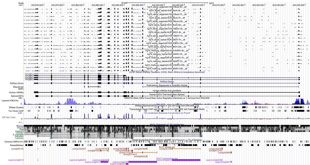
Figure 5: UCSC Genome Browser screenshot of gene TP53BP2.
