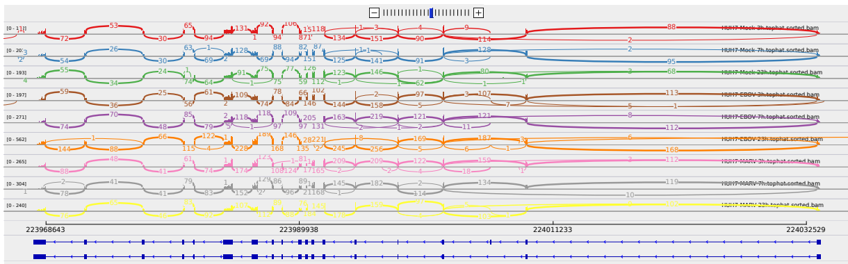
Figure 2: Sashimi plot of gene TP53BP2.
