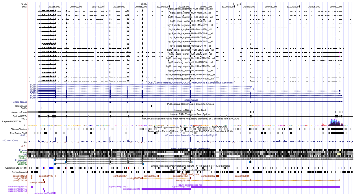
Figure 3: UCSC Genome Browser screenshot of gene SCRIN1.
