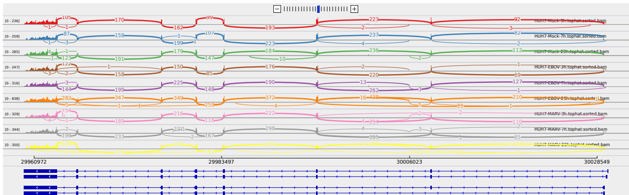
Figure 2: Sashimi plot of gene SCRNI1.
