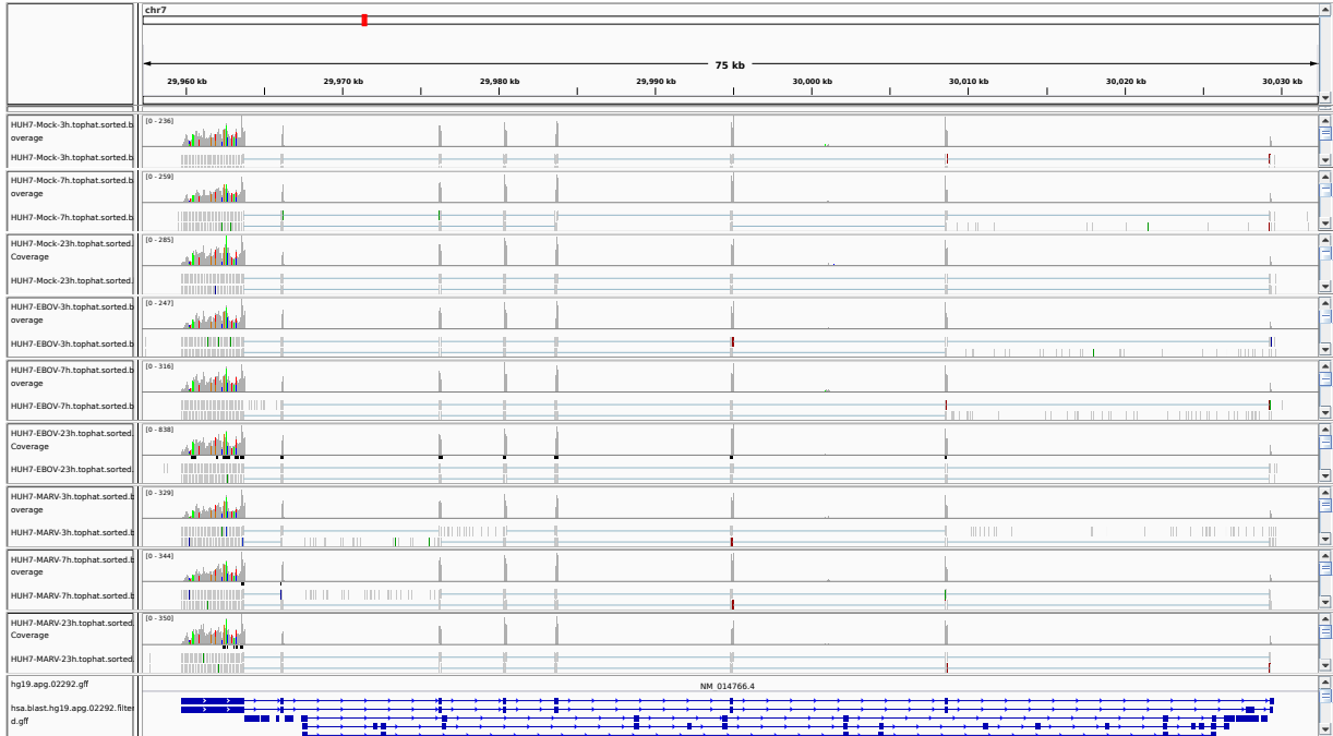
Figure 1: IGV Genome Browser screenshot of gene SCRNI1.
