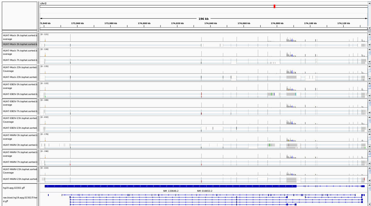
Figure 1: IGV Genome Browser screenshot of gene ZAK.
