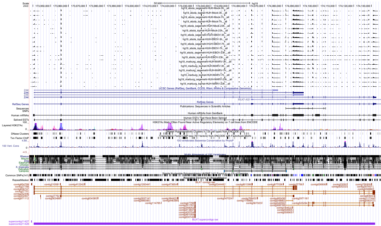
Figure 5: UCSC Genome Browser screenshot of gene ZAK.
