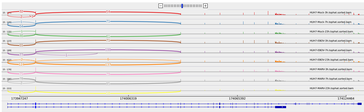
Figure 3: Sashimi plot of gene ZAK.
