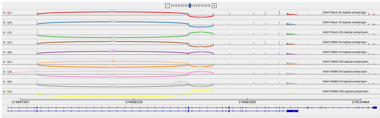
Figure 4: Sashimi plot of gene ZAK.
