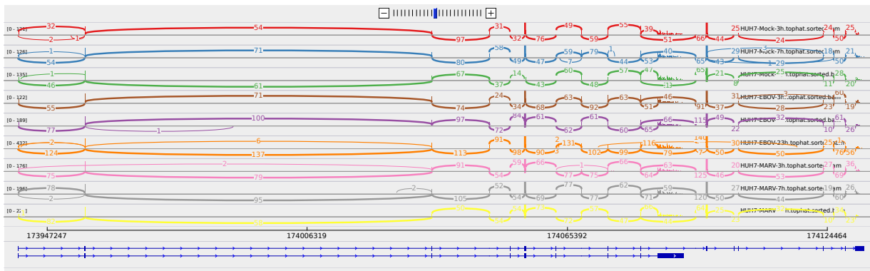
Figure 2: Sashimi plot of gene ZAK.
