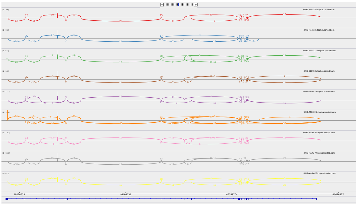
Figure 2: Sashimi plot of gene AMBRA1.
