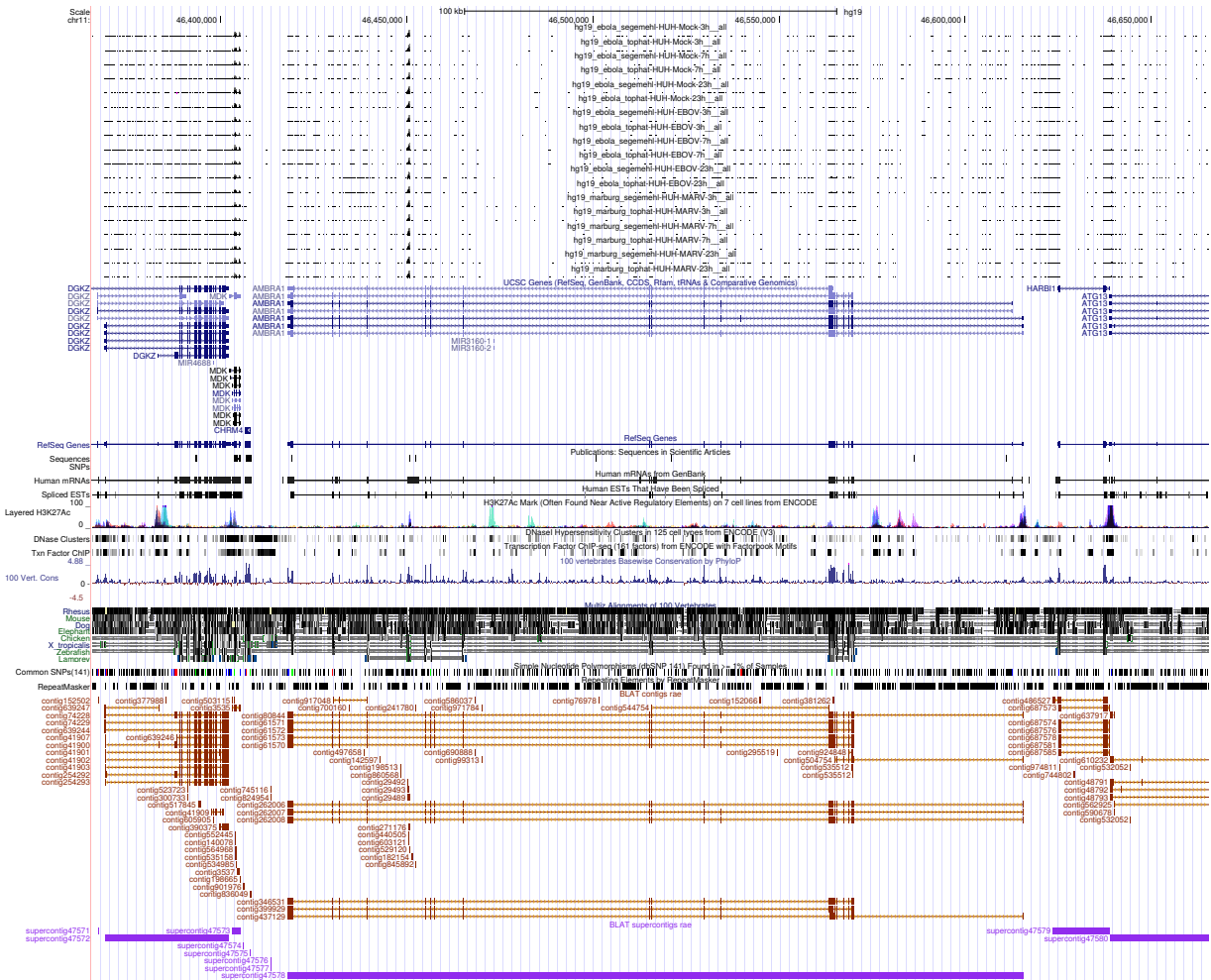
Figure 3: UCSC Genome Browser screenshot of gene AMBRA1.
