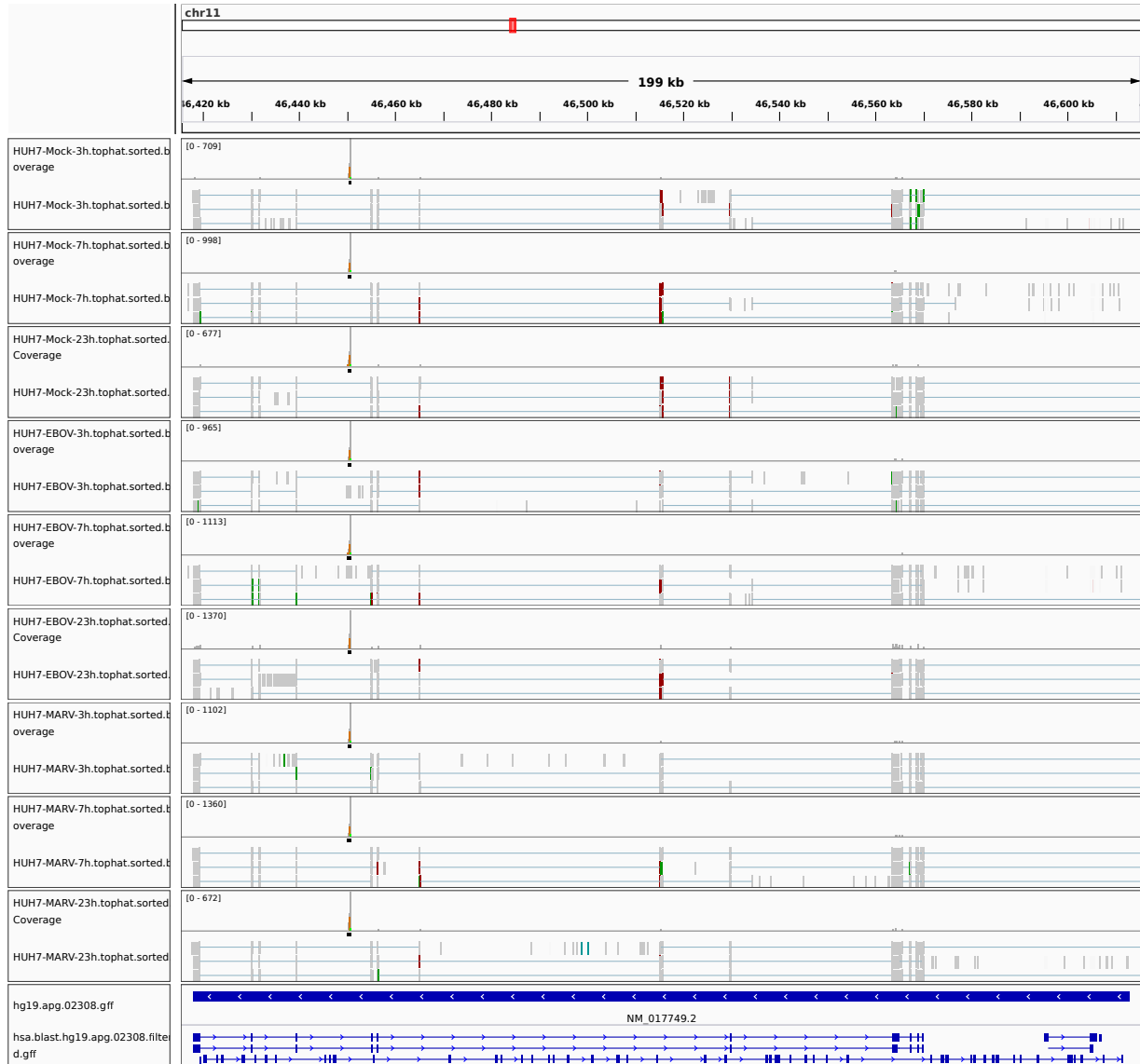
Figure 1: IGV Genome Browser screenshot of gene AMBRA1.
