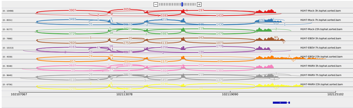
Figure 2: Sashimi plot of gene LOC100652751.
