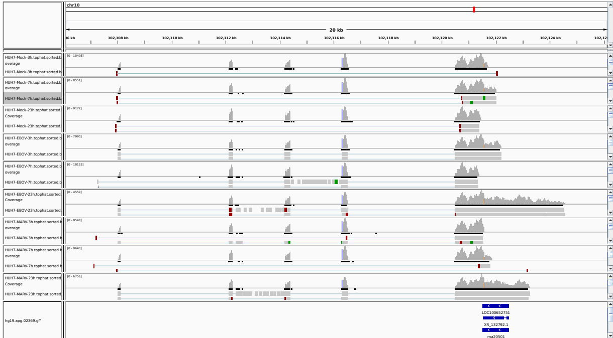
Figure 1: IGV Genome Browser screenshot of gene LOC100652751.
