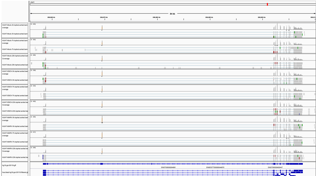
Figure 1: IGV Genome Browser screenshot of gene MAPKAPK2.
