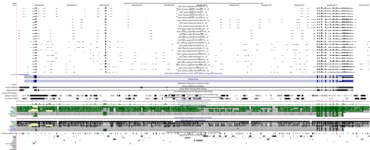
Figure 3: UCSC Genome Browser screenshot of gene MAPKAPK2.
