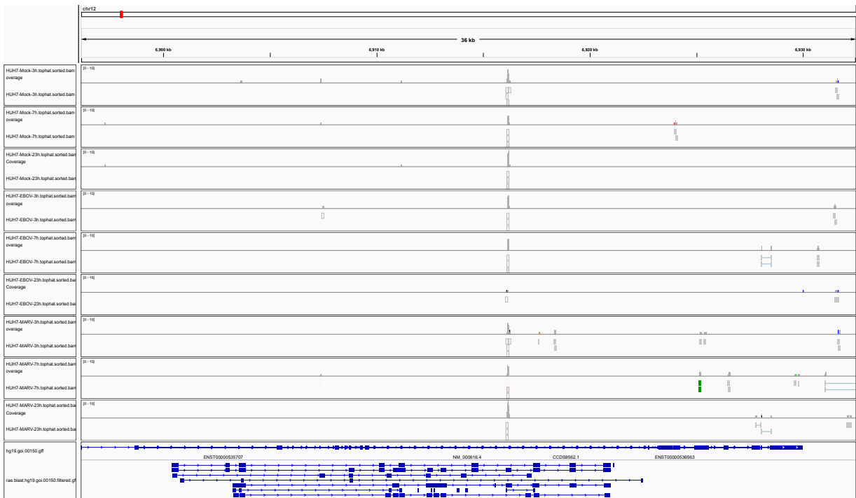
Figure 1: IGV Genome Browser screenshot of gene CD4.
