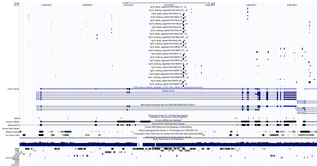
Figure 3: UCSC Genome Browser screenshot of gene CD4.
