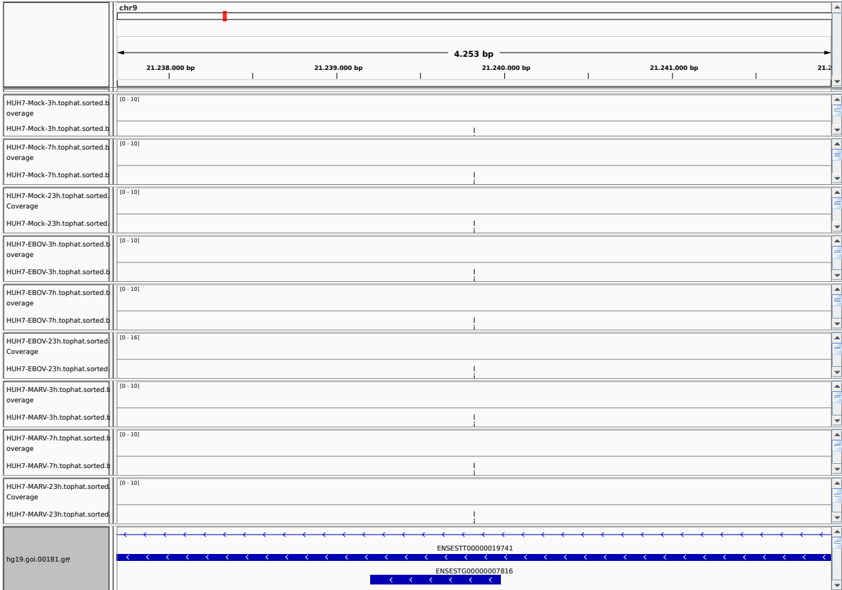
Figure 1: IGV Genome Browser screenshot of gene IFNA14.
