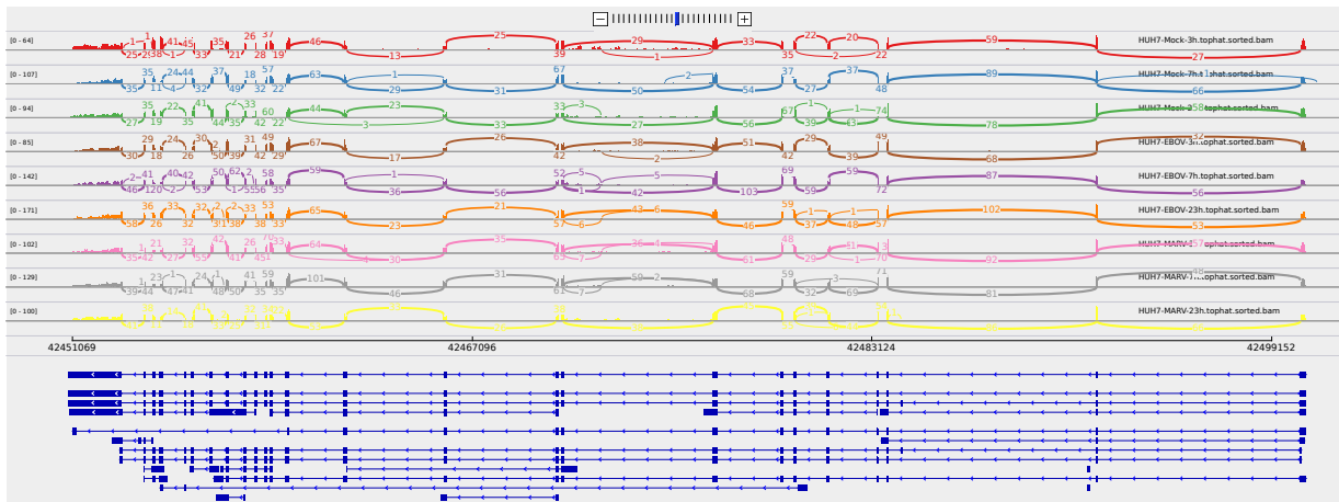
Figure 2: Sashimi plot of gene VPS39.
