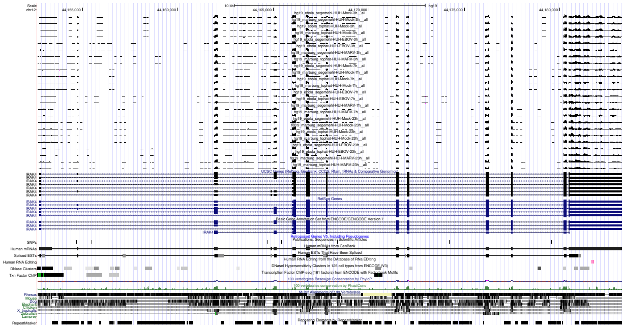
Figure 3: UCSC Genome Browser screenshot of gene VPS39.
