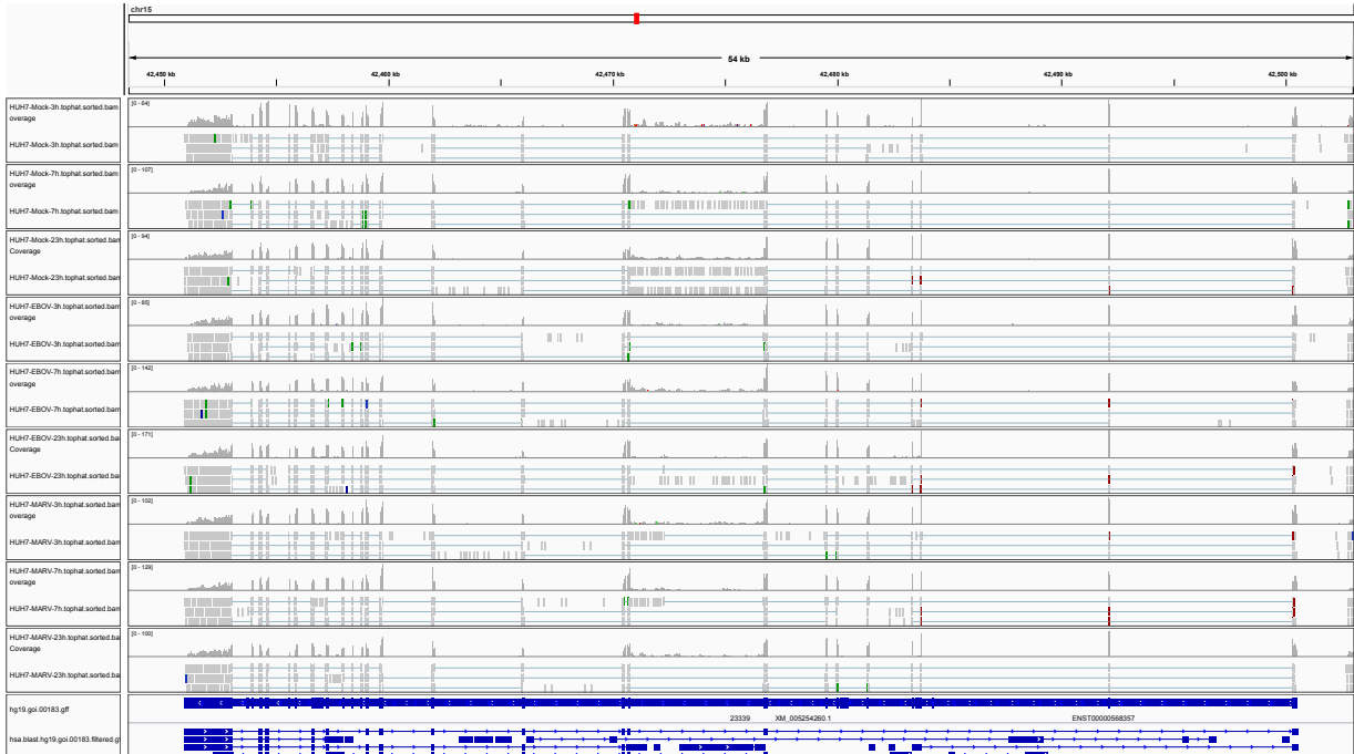
Figure 1: IGV Genome Browser screenshot of gene VPS39.
