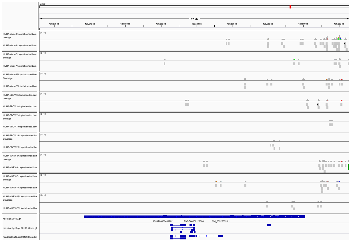
Figure 1: IGV Genome Browser screenshot of gene IRF5.
