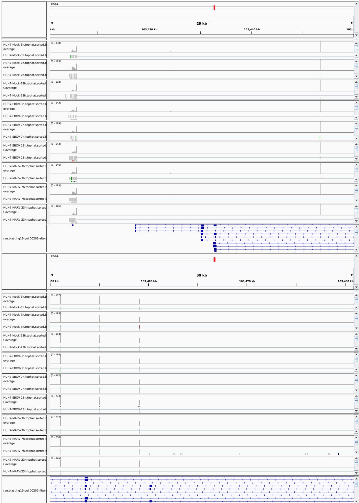
Figure 1: IGV Genome Browser screenshot of gene NFKB1. No changes of expressions rates and patterns between datasets.
