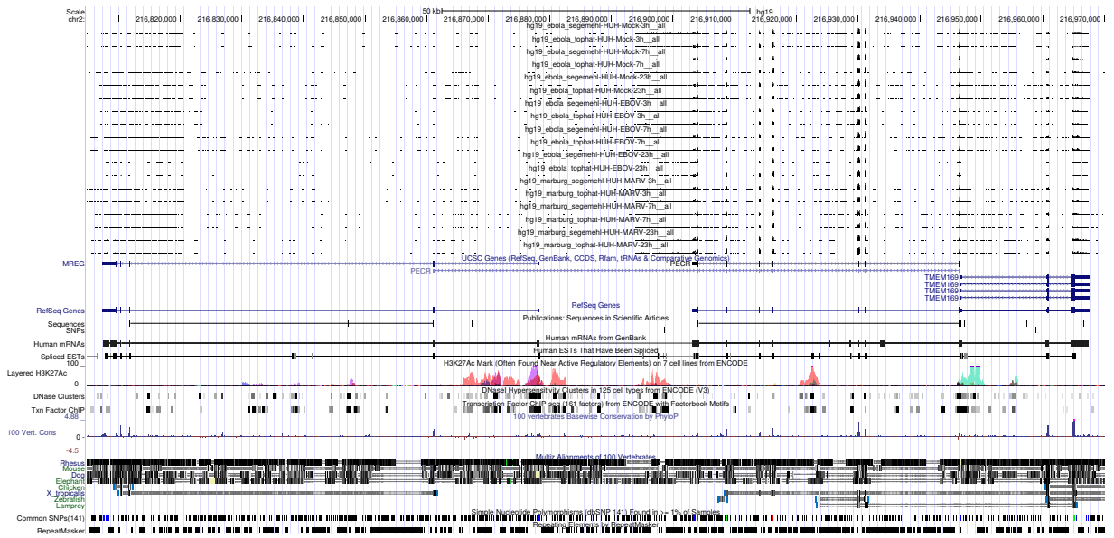
Figure 3: UCSC Genome Browser screenshot of gene PECR.
