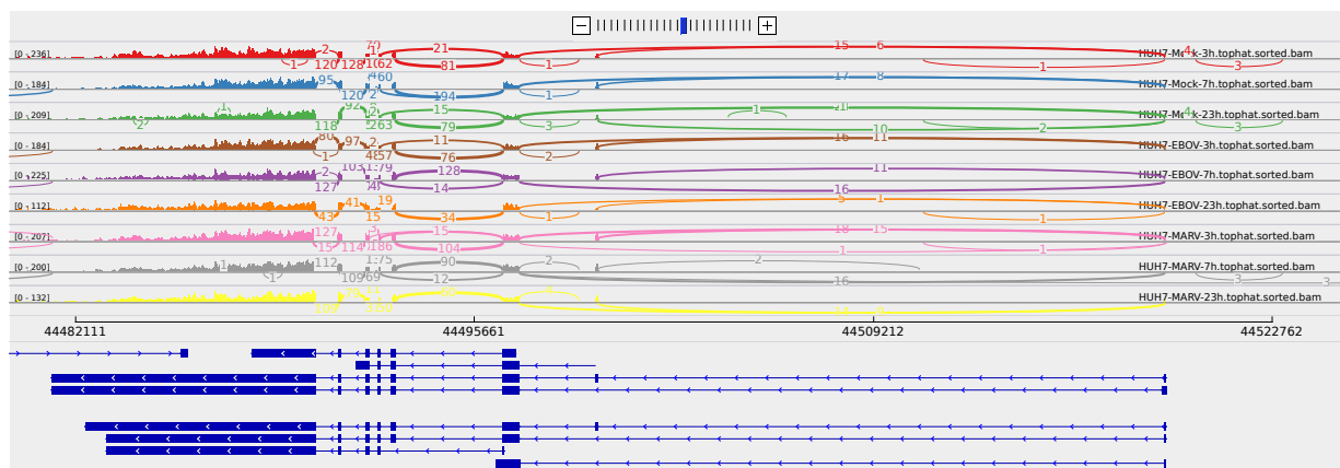
Figure 2: Sashimi plot of gene ZNF445.
