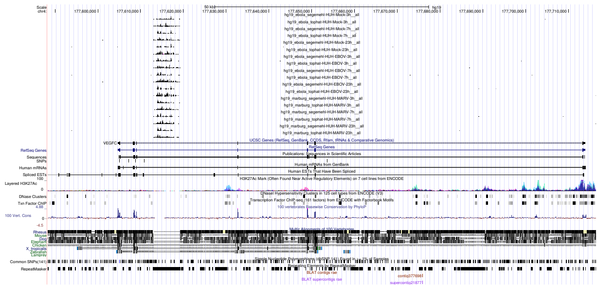
Figure 3: UCSC Genome Browser screenshot of gene VEGFC.
