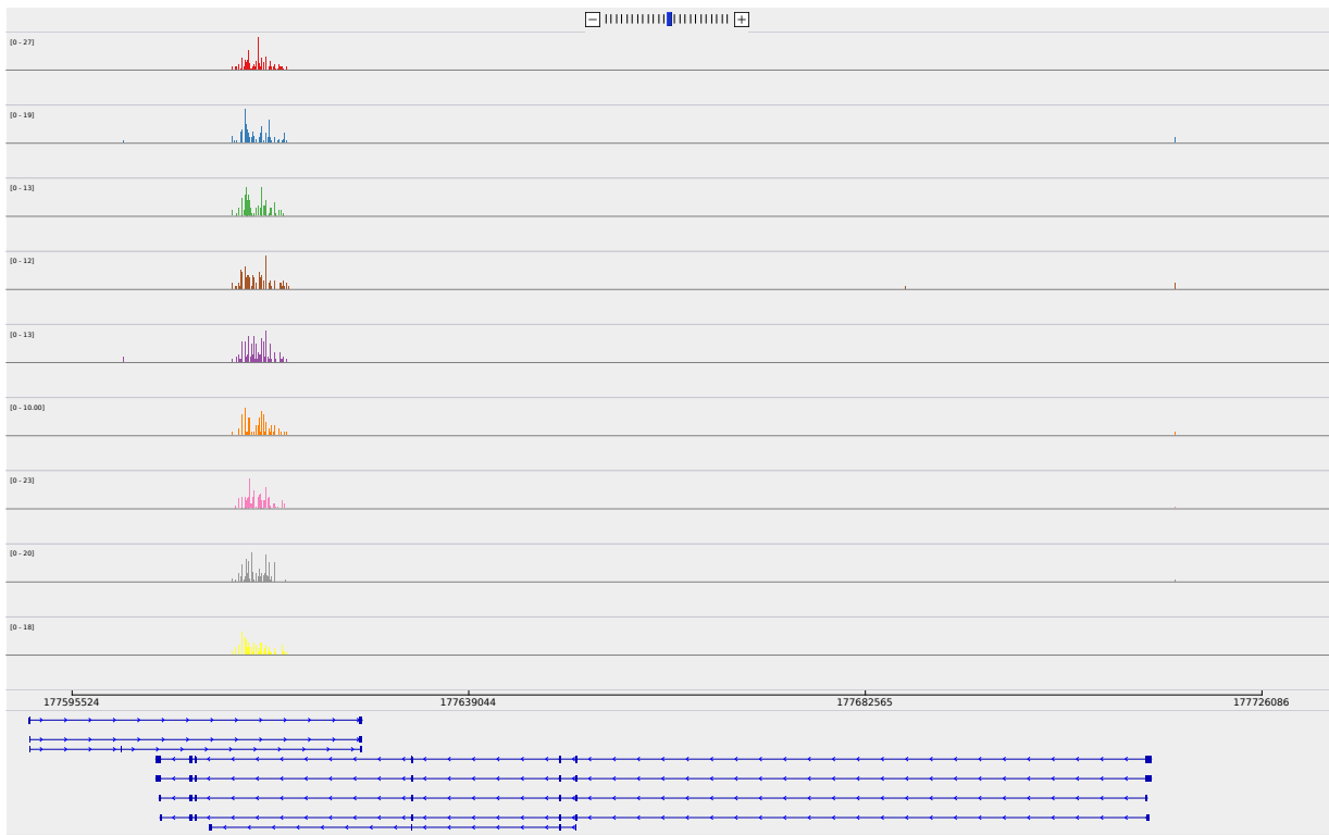
Figure 2: Sashimi plot of gene VEGFC.
