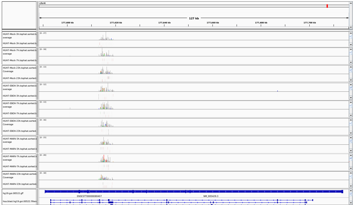
Figure 1: IGV Genome Browser screenshot of gene VEGFC.
