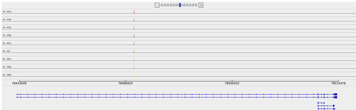
Figure 2: Sashimi plot of gene CXCL13.
