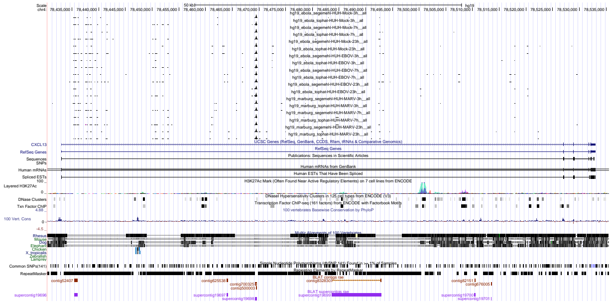
Figure 3: UCSC Genome Browser screenshot of gene CXCL13.
