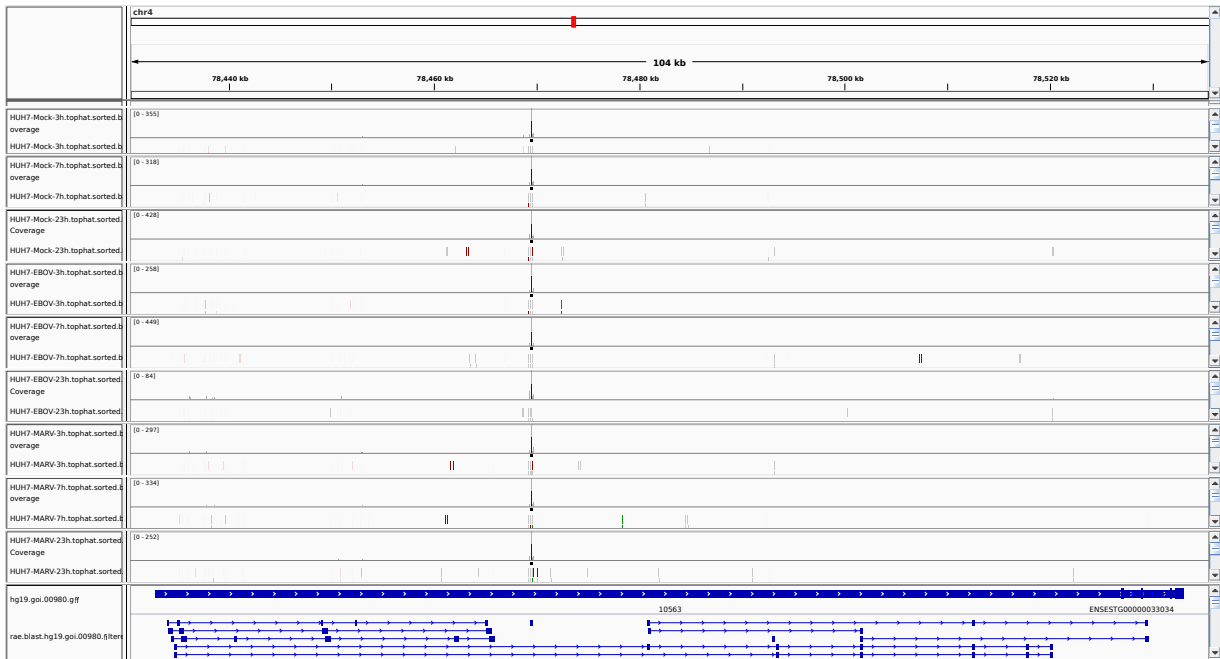
Figure 1: IGV Genome Browser screenshot of gene CXCL13.
