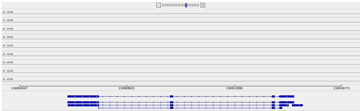
Figure 2: Sashimi plot of gene CXCL14.
