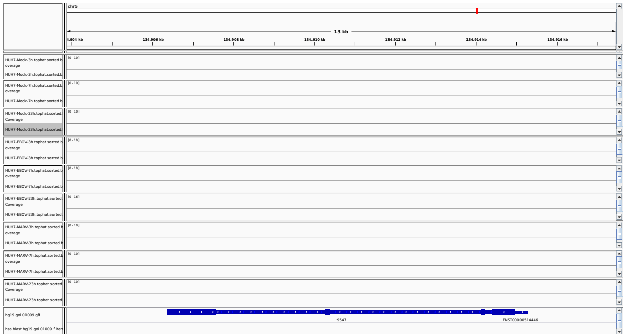
Figure 1: IGV Genome Browser screenshot of gene CXCL14.
