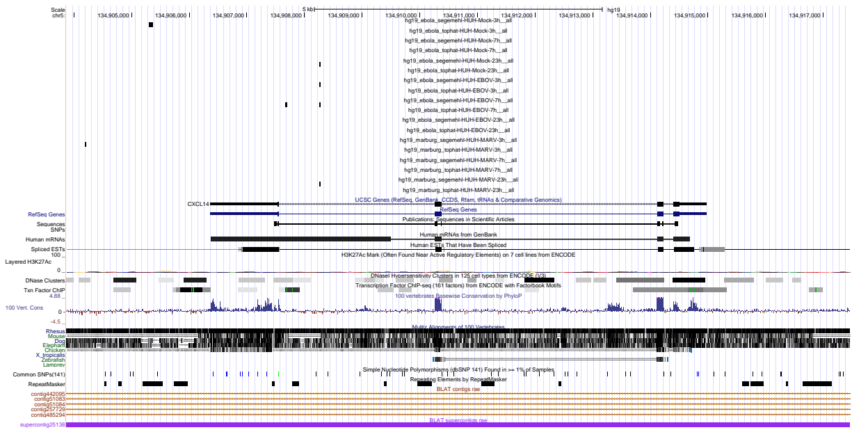
Figure 3: UCSC Genome Browser screenshot of gene CXCL14.
