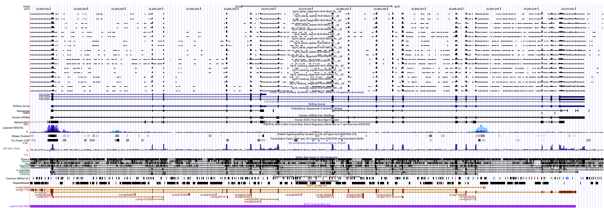
Figure 3: UCSC Genome Browser screenshot of gene PDCD6IP.
