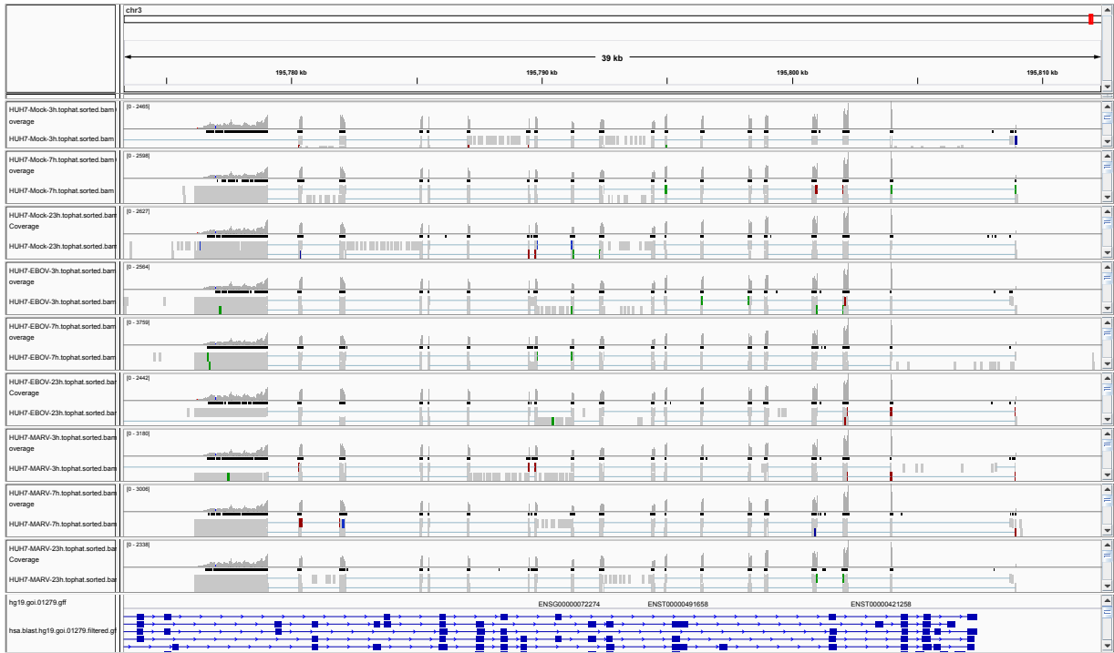
Figure 1: IGV Genome Browser screenshot of gene TFRC.
