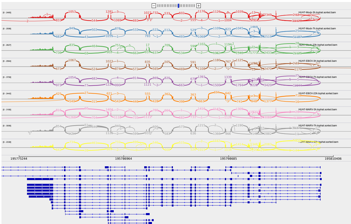
Figure 2: Sashimi plot of gene TFRC.
