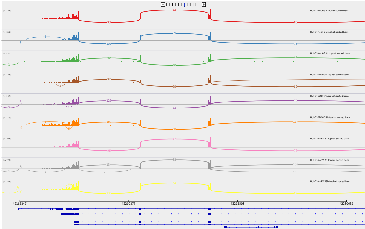
Figure 2: Sashimi plot of gene EHD4.
