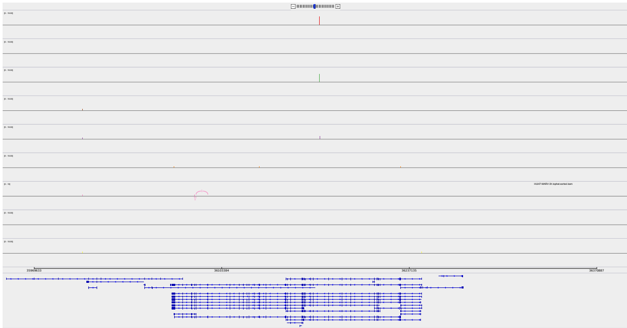
Figure 2: Sashimi plot of gene ARAP2.
