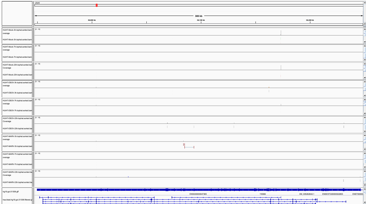
Figure 1: IGV Genome Browser screenshot of gene ARAP2.
